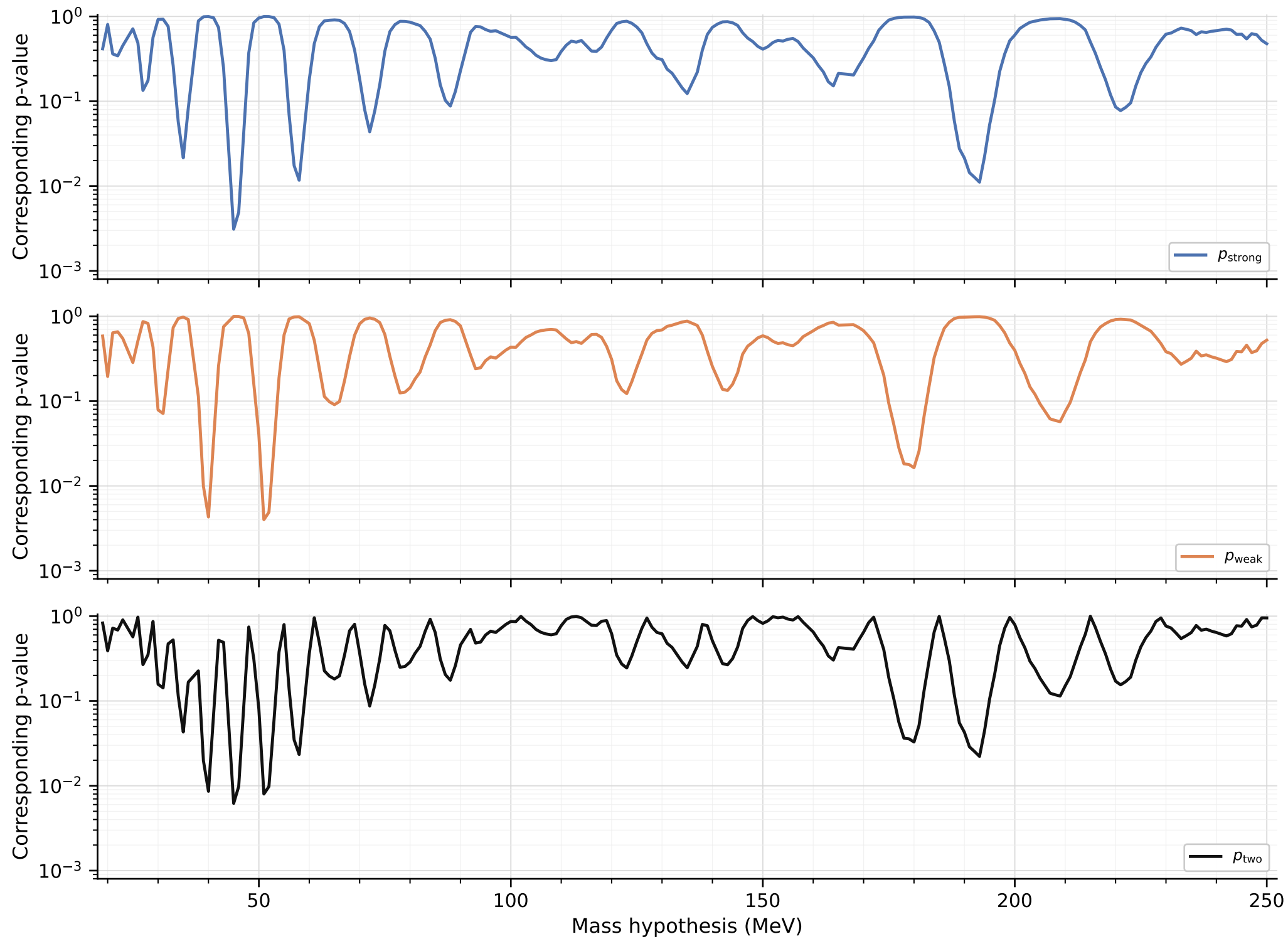
Upper-limit consistency p-values from background-only toys
