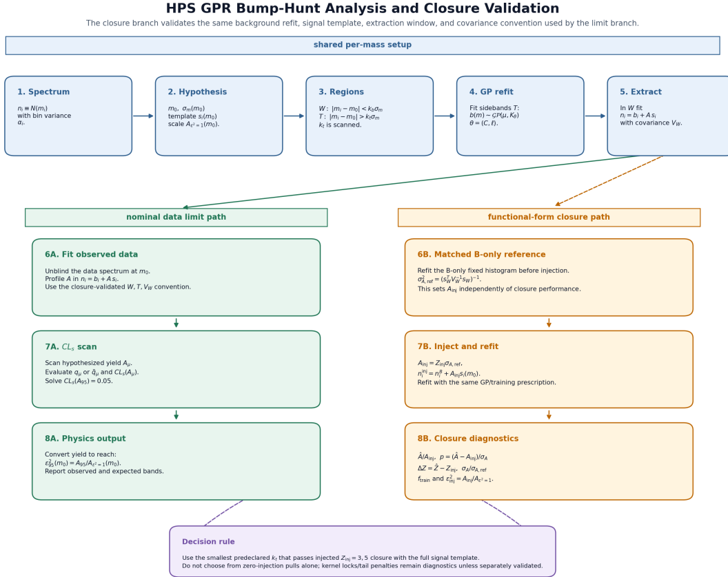
Figure 41: Analysis and validation flow. In the data path, sidebands around each mass hypothesis train the GP and the blinded bins enter the signal-plus-background likelihood. In the validation path, a smooth source-fitted mean is Poisson fluctuated, a known signal may be added, and the complete GP fit and extraction are repeated. The zero-injection ensemble tests spurious signal; nonzero injections test signal recovery and uncertainty calibration. These are extraction-closure tests, not confidence-limit coverage or a scan-wide significance calibration.
