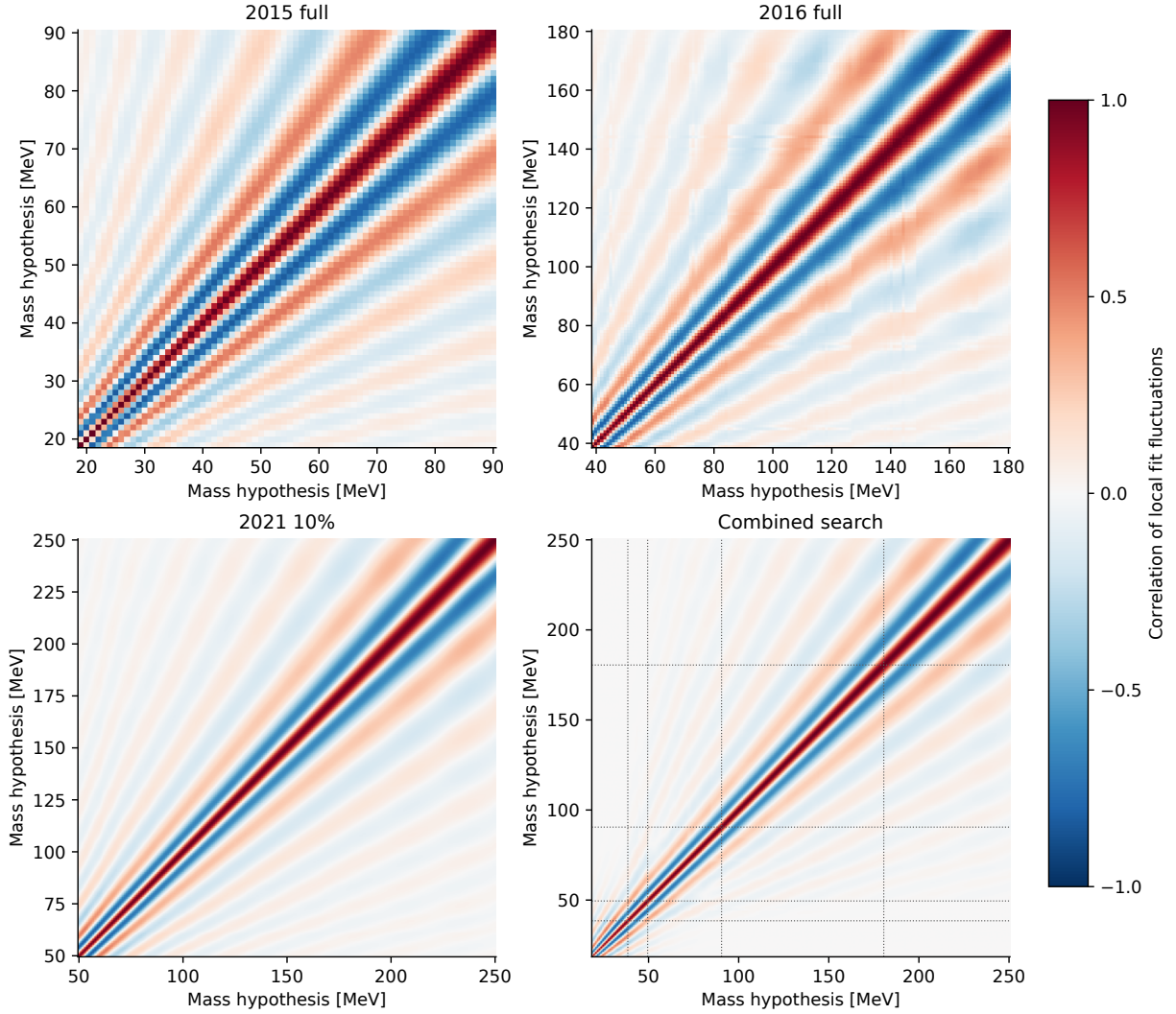
Figure 77: Profiled-response correlation matrices under the archived generating backgrounds: 2015 full at top left, 2016 full at top right, 2021 10% at bottom left, and the combined search at bottom right. All four panels use the same dimensionless color scale. Positive and negative entries describe same-direction and opposite-direction statistical fluctuations. Dotted lines in the combined panel mark changes in the active datasets. The matrices quantify dependence; they do not assign a probability to a selected observed echo or describe correlations of physical signal production.
