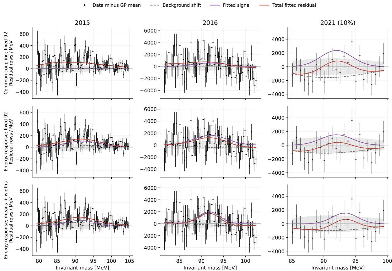
Figure 158: The same observed residuals under common coupling, an energy-dependent rate, and additional shape freedom. The profiled background adjustment remains visible alongside the signal contribution. These are alternative descriptions of the same selected data.
