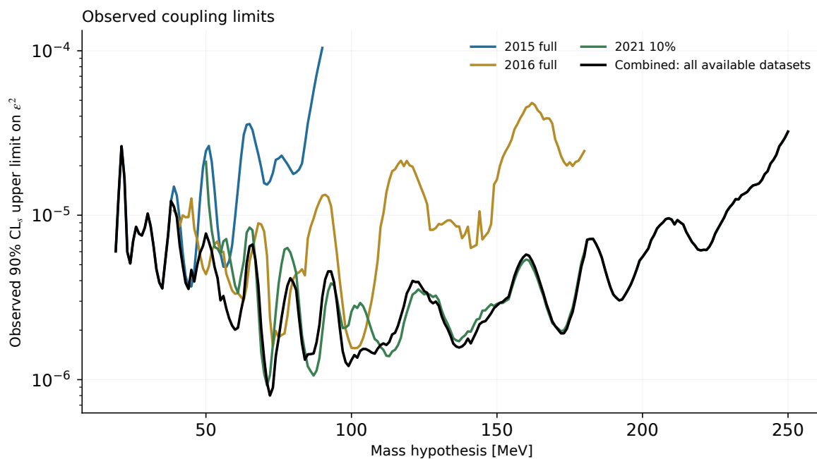
Figure 129: Historical parent Figure 53: observed coupling overlay. This saved display uses the former 2015 endpoint of 90 MeV. The corresponding result retained in v5.0.5 is Figure 55.
