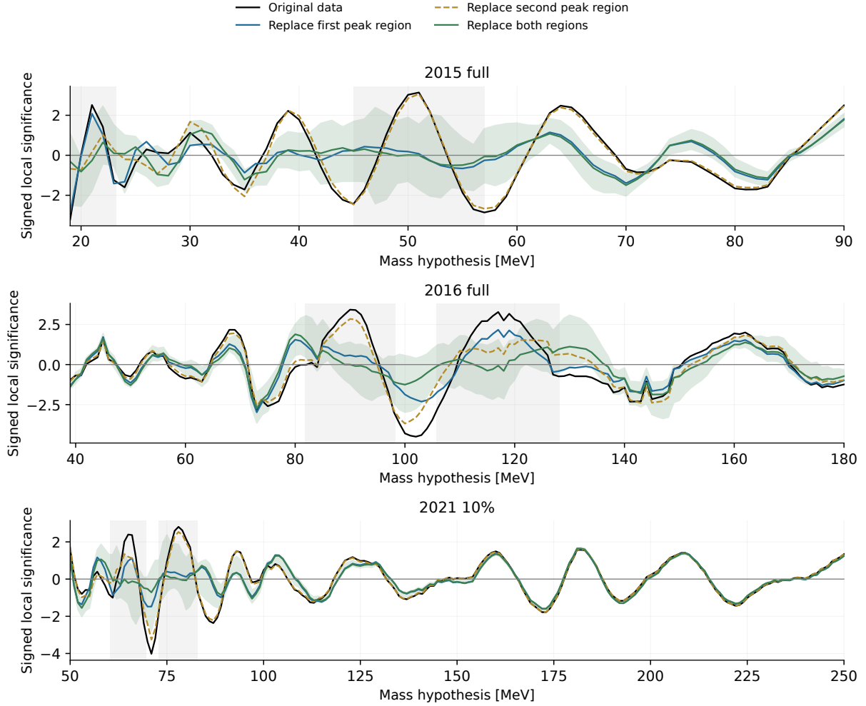
Figure 79: Observed scans before and after conditional replacement of the two selected candidate regions in each year. The first and second regions are, respectively, 45–57 and 18.75–23.25 MeV in 2015 (centers 51 and 21 MeV); 81.75–98.25 and 105.75–128.25 MeV in 2016 (90 and 117 MeV); and 72.875–82.875 and 60.375–69.75 MeV in 2021 (78 and 65 MeV). Boundaries follow the stored whole-bin selections around the 2.25\sigma_m masks. The envelope spans ten conditional replacements and is not a confidence band. Changes demonstrate how the local fit responds to altered candidate bins; the untouched remote variation is quantified in Appendix E. All curves retain their existing tested masses and the same nominal local-significance mapping.
