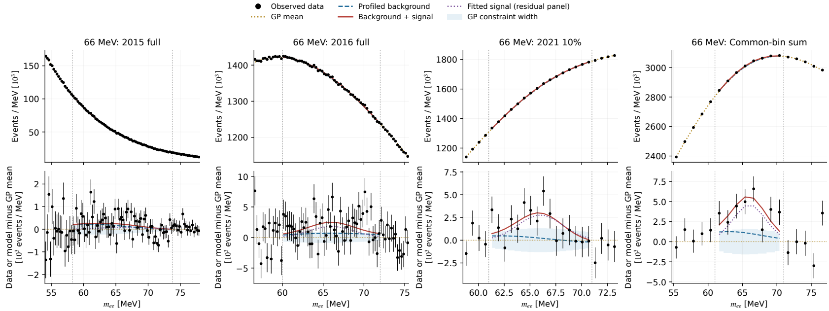
Figure 69: Common-coupling extraction at 66 MeV, with a shared fitted amplitude \hat{\epsilon}^2 = 4.55 \times 10^{-6} and nominal local significance 2.76. Each campaign retains its own yield conversion and resolution. Bars show counting error only. Colored shading in the residuals is the zero-centered GP constraint width; it is neither fitted-background uncertainty nor total residual uncertainty.
