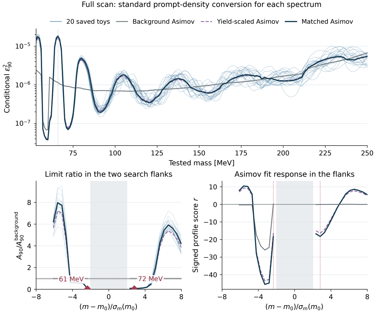
Figure 150: Historical 1%-based injection at 66 MeV, scaled to full exposure. The selected count-limit minima at 61 and 72 MeV have reductions of 92.9% and 92.2% relative to the scenario's continuum-only Asimov limits; 61 MeV is a flank endpoint.
