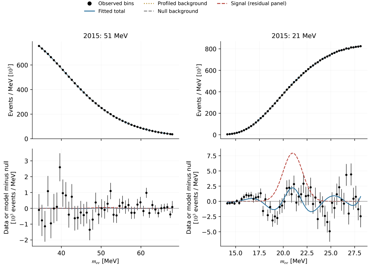
Figure 108: Traditional baseline fits to full 2015 data. At 51 and 21 MeV the nominal local coordinates are 0.131 and 5.580, with D/\text{dof} = 141.69/131 and 92.50/50 . Adjacent bins are summed for display: 0.75 MeV at the 51 MeV hypothesis, and 0.25 MeV at 21 MeV. Every fit still uses the original 0.25 MeV bins. Counts and residuals are divided by the actual displayed width, including a partial endpoint group. Bottom: data minus the refitted null background, with counting errors only. The red Gaussian is not the blue total change: the polynomial background also moves. Subtraction induces correlated residuals. The large 21 MeV root accompanies an inadequate overall fit. Table 23 retains all variants, including the badly fitting degree-two model at 51 MeV; neither extreme is a defensible physical significance.
