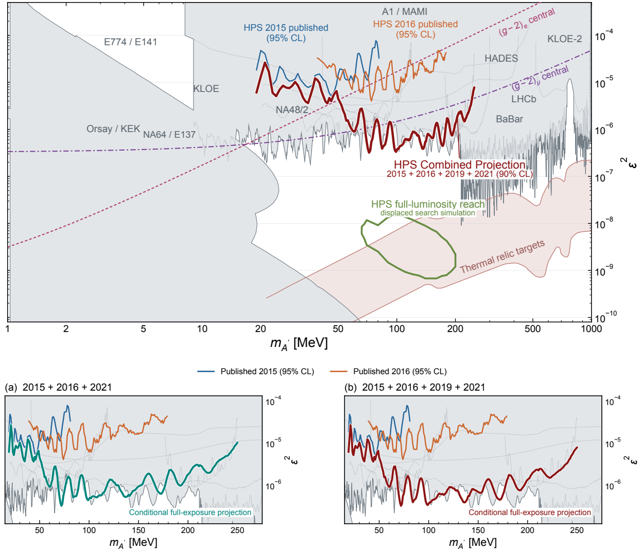
Figure 2: Visible dark-photon parameter space. Top: archived exclusions, published HPS 2015 and 2016 limits (95% CL), the four-campaign prompt projection (90% CL), and the poster’s simulated displaced full-luminosity reach. The gray contours and thermal target are historical context, rather than a complete 2026 survey; their sources and display conventions are listed in Appendix L. Lepton-anomaly lines show central-value references only: \Delta a_\mu = 38 \times 10^{-11} (compatible with zero) and \Delta a_e \simeq 0.34 \times 10^{-12} [5, 6, 7]. (a) 2015+2016+2021; (b) 2015+2016+2019+2021. The prompt projections preserve the current-sample structure and apply statistics-only density scaling to full exposure. The 2019 dataset is a nominal 1% sample with a 2021-response proxy. These curves are conditional observed-equivalent projections; they are not expected sensitivity curves or observed full-data exclusions.
