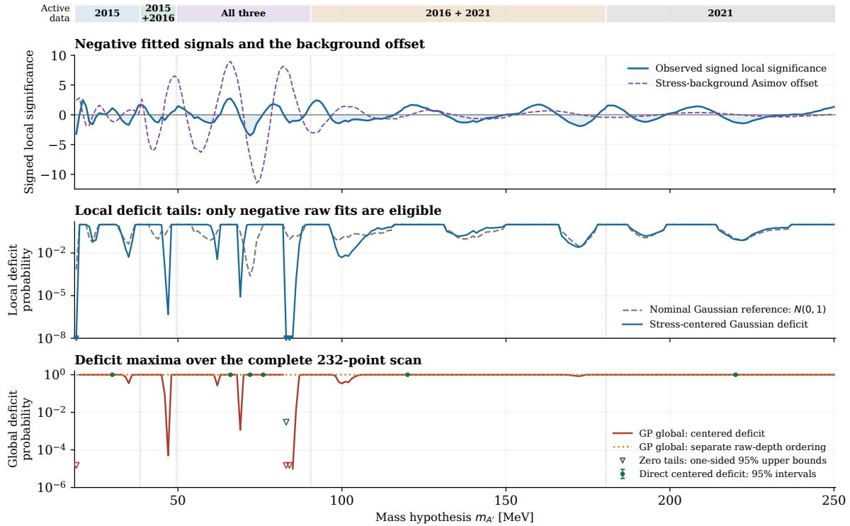
Figure 111: Profiled deficit scan. Top: observed signed local significance and the stress-background offset; shading marks negative fitted contributions. Middle: raw-root Gaussian reference and conditional Gaussian-response tails. Both assign one to nonnegative raw roots. Local triangles mark the 10^{-8} display floor. Bottom: two separate global orderings; triangles mark one-sided 95% zero-count bounds. Direct error bars are central 95% intervals.
