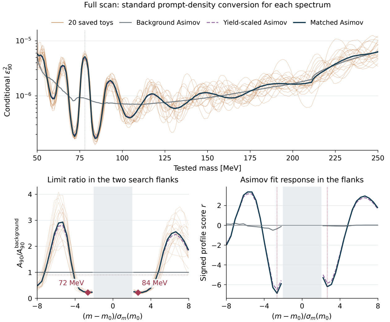
Figure 89: The corresponding 78 MeV example. A central excess can accompany lower upper limits on either side as its counts enter neighboring GP training regions.
