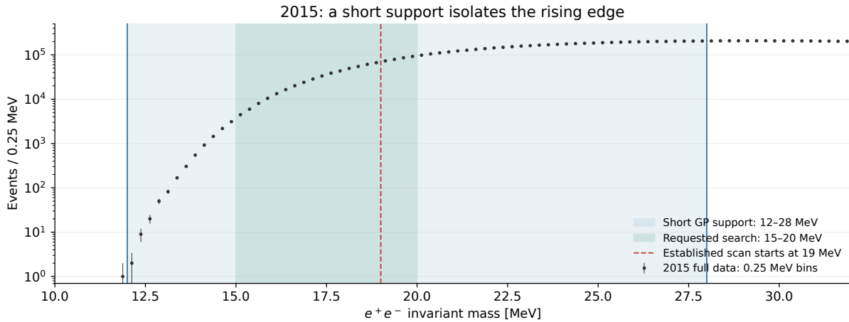
Figure 145: The same released full-2015 histogram, summed from 0.05 to 0.25 MeV bins. The chosen GP support is 12–28 MeV; the requested search is 15–20 MeV. The dashed line marks the lower boundary of the established scan, not the lower boundary of the available counts.
