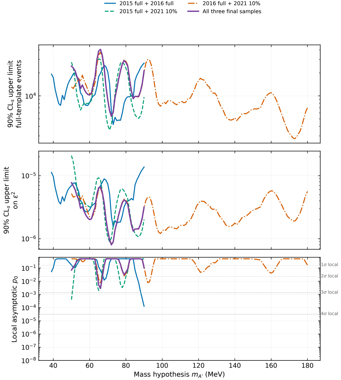
Figure 132: Historical parent Figure 58: combined final results. This saved display uses the former 2015 endpoint of 90 MeV. The corresponding result retained in v5.0.5 is Figure 60.
