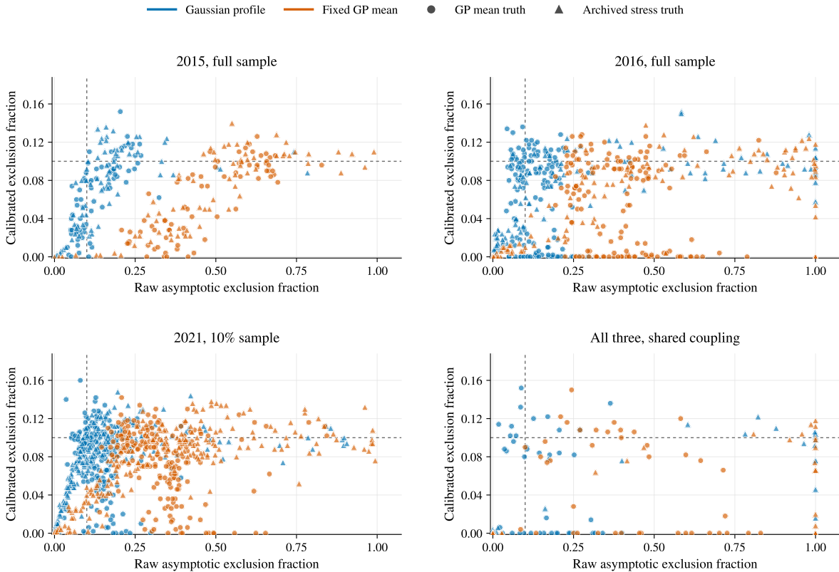
Figure 105: Independent validation with five-reference-error injections. The horizontal coordinate is the fraction of 500 spectra excluding the known injected yield with the raw asymptotic rule; the vertical coordinate uses the calibrated two-truth envelope. A point far to the right has an excessive raw exclusion rate. A point below the horizontal 0.10 guide indicates a conservative calibrated rate in that cell. The guides mark the nominal benchmark, not an expected discovery probability. Finite counts and Monte Carlo uncertainty limit the precision of each conclusion.
