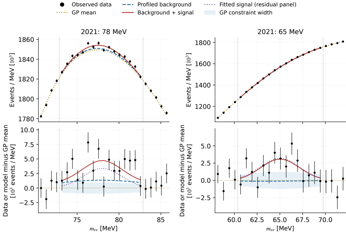
Figure 74: The leading separated excesses in the released 2021 10% sample at 78 and 65 MeV. These masses are fixed by the existing observed scan and are distinct from the combined 66 MeV coordinate. Bars show counting error only; residual shading shows the zero-centered GP constraint width, not fitted-background or total residual uncertainty.
