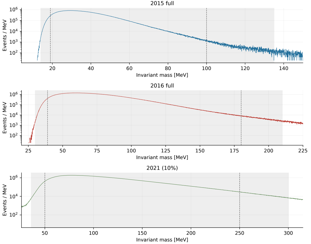
Figure 7: Invariant-mass distributions for the 2015, 2016 and 2021 datasets, shown in events per MeV with original bin widths of 0.05, 0.05 and 0.125 MeV, respectively. Gray shading marks the current GP supports, including 36–300 MeV for 2021, and dashed lines bound the narrower interval in which signal hypotheses are tested. The mass-dependent 2.25\sigma_m exclusion is removed from the GP support separately at every tested mass.
