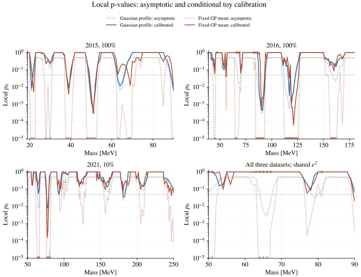
Figure 103: Asymptotic local probabilities and the larger background-only tail from the two calibration truths. The empirical bounded-statistic convention gives one when the discovery statistic is zero; the earlier asymptotic display gives 0.5. Triangles retain asymptotic values below the plotting floor. Open circles flag limited Monte Carlo precision or a noisy estimate displayed at one; the saved numerical results retain unclipped values. No curve in this figure includes a global trials correction.
