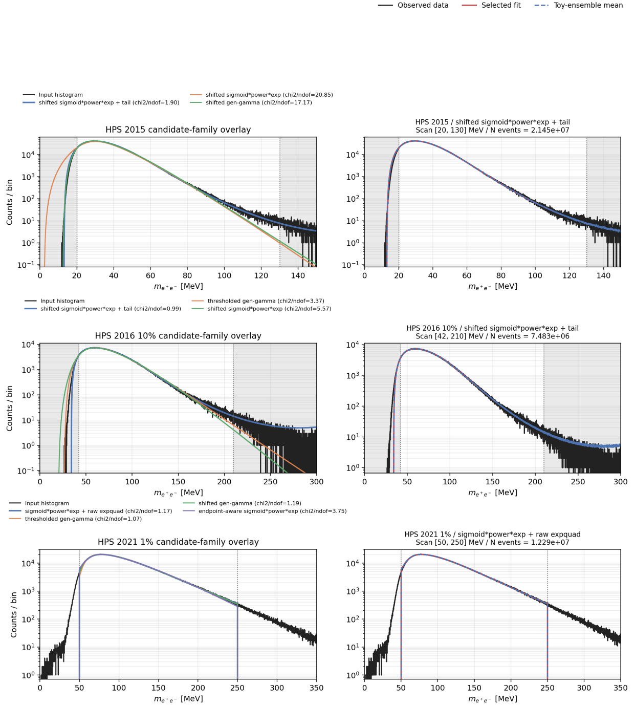
Figure 48: Analytic generating means used in the year-matched functional-form studies. Each dataset row compares the source spectrum with the candidate families and then shows the selected mean against the generated toy ensemble. The functions define smooth positive pseudo-data means and are not asserted to be unique physical models of the continuum.
