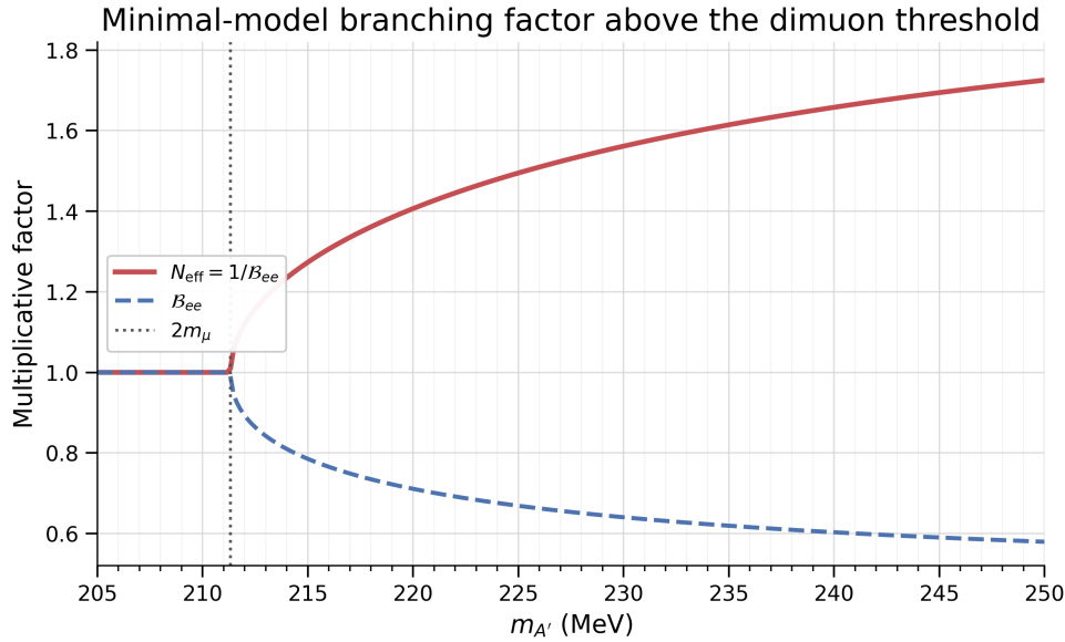
Figure 37: Minimal-model branching factor used to reinterpret electron-channel \varepsilon^2 limits above the dimuon threshold. The red curve shows N_{\text{eff}}^{\text{BR}} = 1/\mathcal{B}(A' \rightarrow e^+e^-) and the blue dashed curve shows \mathcal{B}(A' \rightarrow e^+e^-) .
