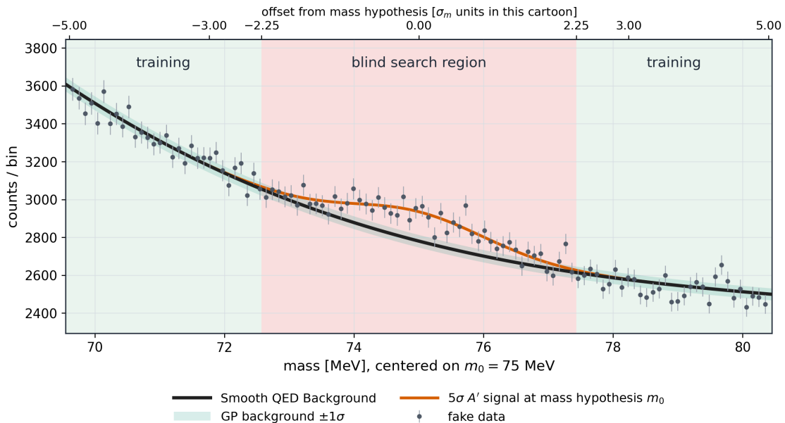
Figure 42: Selected 2.25\sigma_m blind and training-exclusion geometry. The GP is trained outside the widened interval, while all bins inside it enter the local signal-plus-background likelihood. This retains the signal tails for extraction without allowing those same bins to influence the sideband fit.
