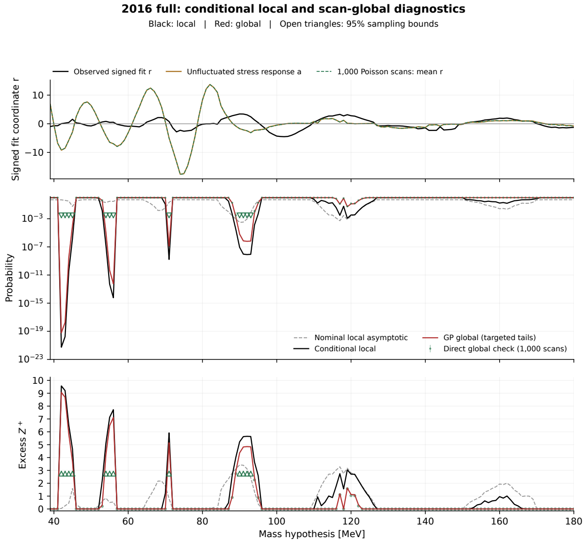
Figure 81: Profiled 2016 conditional global study with the same black-local/red-global convention and integer Z^+ guides. Ordinary sampling uses 2,000,000 fields; targeted importance sampling resolves the previously empty Gaussian tails without altering the field model or ordering. At 42 MeV the conditional Gaussian global probability is 6.096 \times 10^{-20} ( Z = 9.067 ), with 0.16% relative Monte Carlo standard error. This extreme value reflects the biased stress reference, not a particle discovery. The direct Poisson check remains 0/1,000, giving only p < 0.002991 ( Z > 2.749 ); its open triangles retain those bounds. Red shading gives sampling intervals, not background-model uncertainty. This global calculation is different from the Sidak reference. The implementation and stress-reference diagnostics are in Appendix C.
