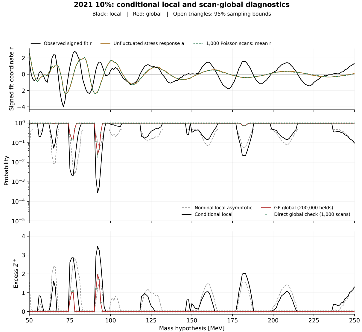
Figure 82: Profiled study for the released 2021 10% sample. The principal ordering selects 92 MeV and gives GP global probability 0.02519 ( Z = 1.957 ), with 26/1,000 direct exceedances. The GP ensemble retains 200,000 fields. Black is the conditional local probability and red the global probability, with the corresponding Z^+ below. This global calculation uses the correlated field rather than the Sidak correction used for the asymptotic references. Qualification of the generating background remains required for a particle-global interpretation. The implementation and stress-reference diagnostics are in Appendix C.
