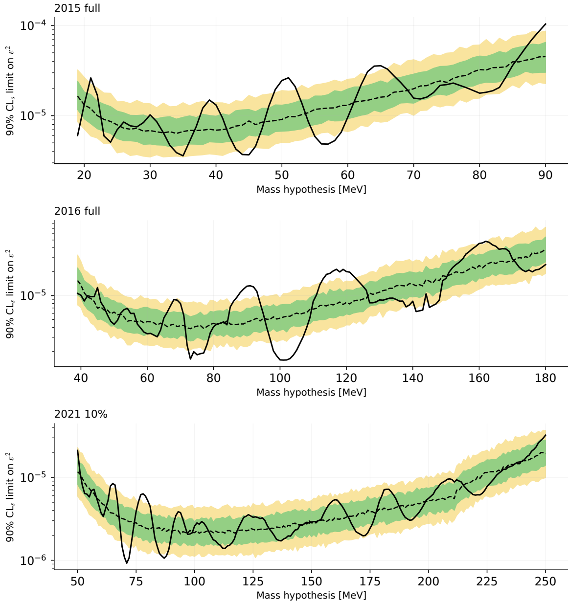
Figure 136: Historical parent Figure 62: individual expected bands. This saved display uses the former 2015 endpoint of 90 MeV. The corresponding result retained in v5.0.5 is Figure 64.
