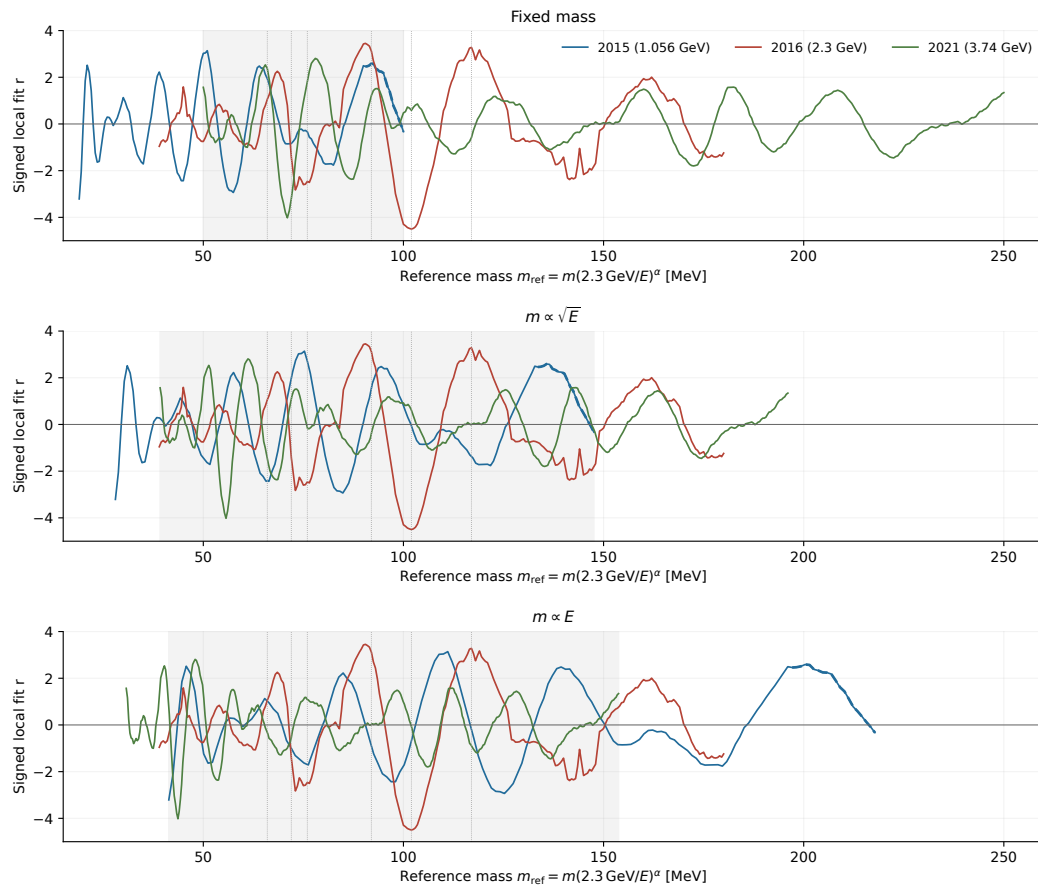
Figure 155: The v5.5.0 scan comparison under fixed, square-root and linear beam-energy mass scaling. The mapped responses test the proposed correspondence between campaigns; their alignment is not evidence for an energy-dependent particle mass.
