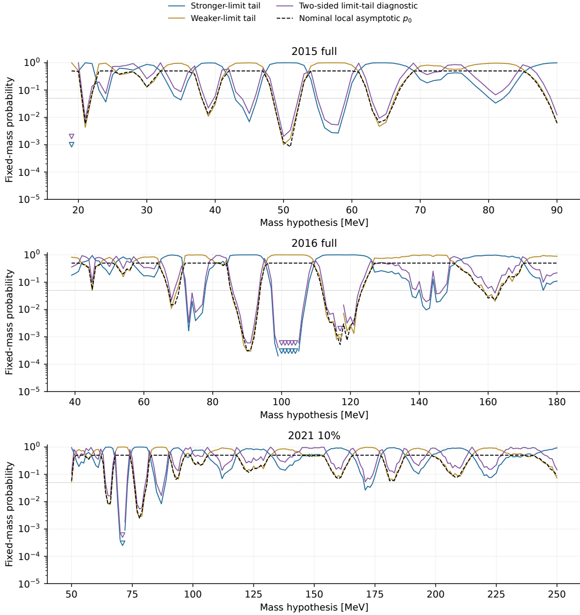
Figure 137: Historical parent Figure 63: individual tail probabilities. This saved display uses the former 2015 endpoint of 90 MeV. The corresponding result retained in v5.0.5 is Figure 65.
