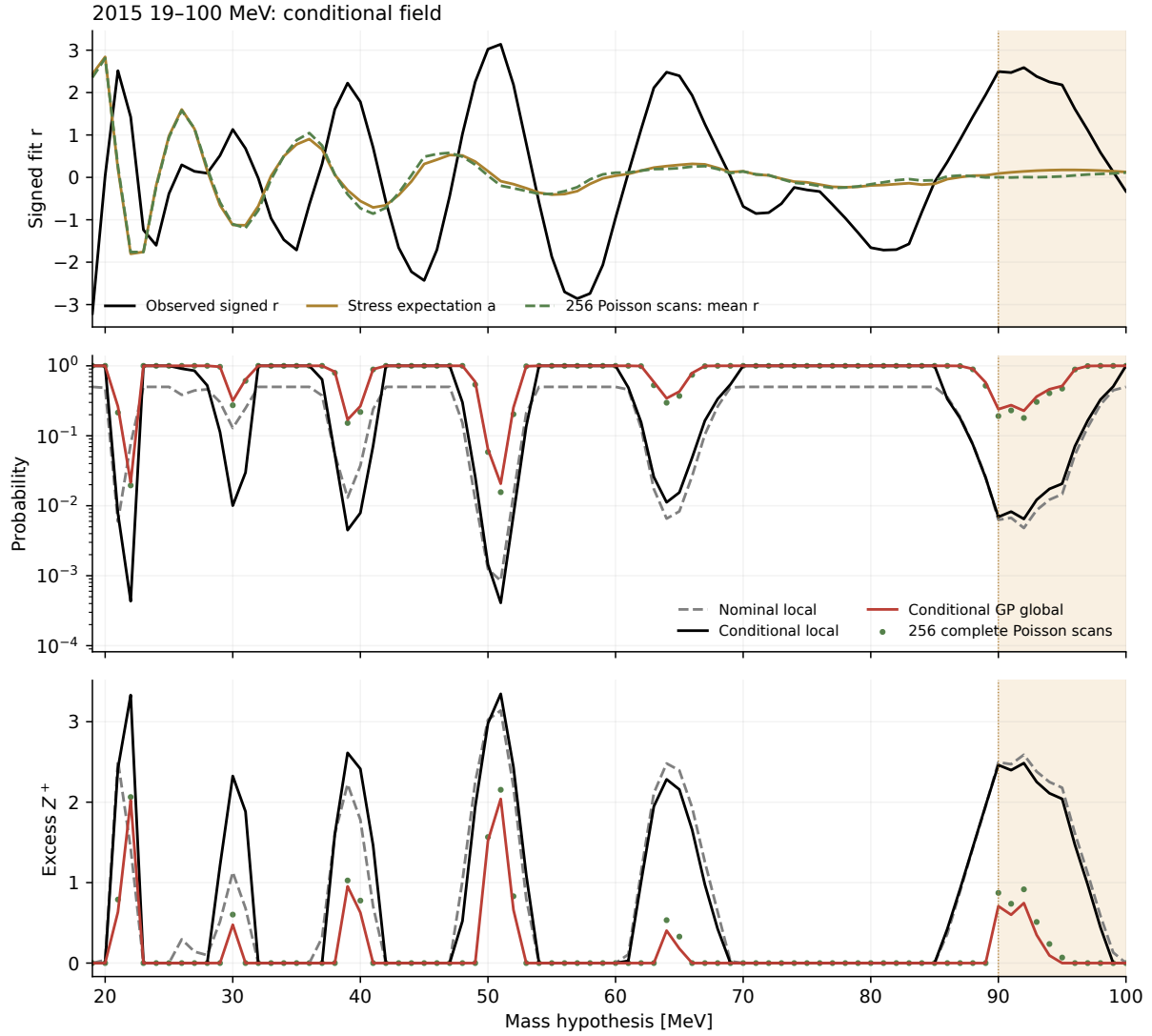
Figure 80: Profiled 2015 conditional local and global probabilities on 19–100 MeV. The full field uses 82 integer hypotheses and the endpoint kernel prescription in Appendix B. Its response matrix and the first 256 coherent Poisson scans are reused from the extended covariance study; 200,000 Gaussian fields integrate the enlarged search. Open symbols retain one-sided 95% bounds for empty direct tails. Probability and Z^+ panels refer to the declared stress model. The interpretation, sigcorr check and sampling method are in Appendix C.
