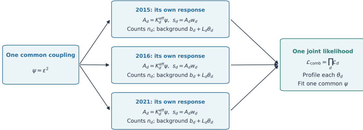
Figure 36: One coupling predicts a campaign-specific signal through its normalization and resolution. Each campaign retains its own counts and correlated background constraint; the likelihoods are multiplied and fitted with one common coupling. Only datasets whose declared search contains the tested mass contribute.
