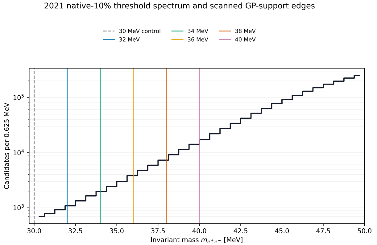
Figure 52: Native 2021 10% source histogram near threshold. Vertical lines mark the 30 MeV control and the five candidate lower edges of the GP support. The logarithmic vertical scale makes the low-count shoulder and rapid turn-on visible.
