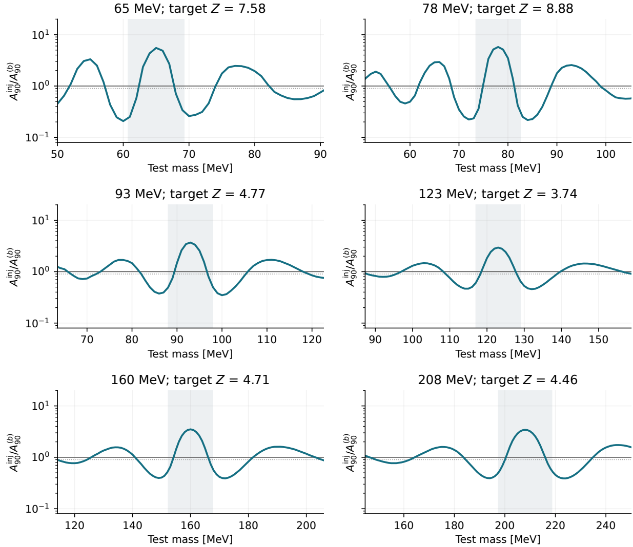
Figure 87: Six alternative injections based on the 10% sample. Curves show the matched-Asimov count-limit ratio in Eq. (113); shaded central intervals mark |m - m_0| < 2\sigma_m , outside the echo search. Each panel uses its own fitted continuum. The alternatives are not a simultaneous six-peak hypothesis.
