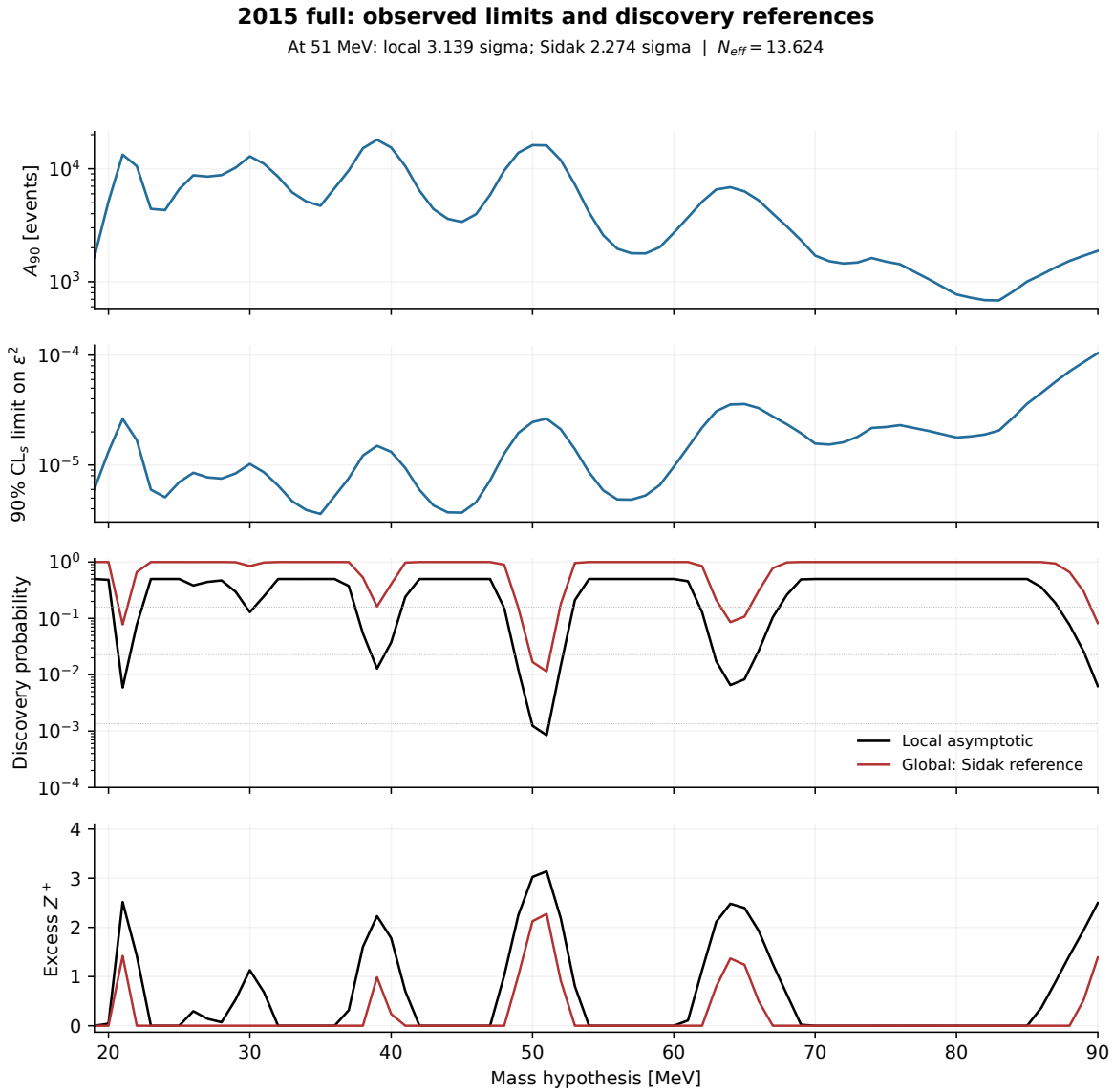
Figure 131: Historical parent Figure 55: observed scan 2015. This saved display uses the former 2015 endpoint of 90 MeV. The corresponding result retained in v5.0.5 is Figure 57.
