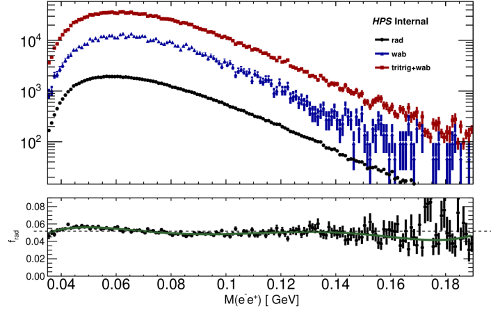
Figure 30: The differential rates in units of \text{MeV}^{-1} for all the MC samples which go into the radiative fraction. The rad component is a function of the true mass of the generator level \gamma^* for the event. The WAB and tritrig components are a function of the invariant mass of the selected V0 candidate. The bottom panel shows the radiative fraction, the green line is the fifth order polynomial fit, and the dotted line is the zeroth order polynomial fit.
