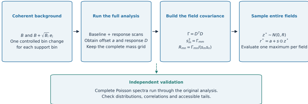
Figure 40: The computational gain in the significance-GP method. Full analysis scans of controlled perturbations estimate the field covariance once. Gaussian vector draws then produce many correlated scans without repeating those fits. A separate ensemble of complete Poisson experiments tests the approximation. This is an explanatory diagram of the archived HPS implementation, following Ref. [29]; the offset and width are retained explicitly.
