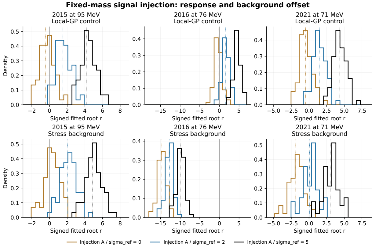
Figure 94: Fixed-mass Poisson injection examples under local GP controls (top) and the archived stress truth (bottom). Each curve uses 64 experiments, paired across the three strengths within a mass and truth. Dotted lines show fits to unfluctuated expectations. The horizontal axis is the signed fitted root; the labels A/\sigma_{\text{ref}} = 0, 2, 5 specify injected yields, not achieved significances. The same reference uncertainty is used for both truths at a fixed mass. Persistent stress offsets are especially clear at 2016 76 MeV. No global discovery efficiency is assigned.
