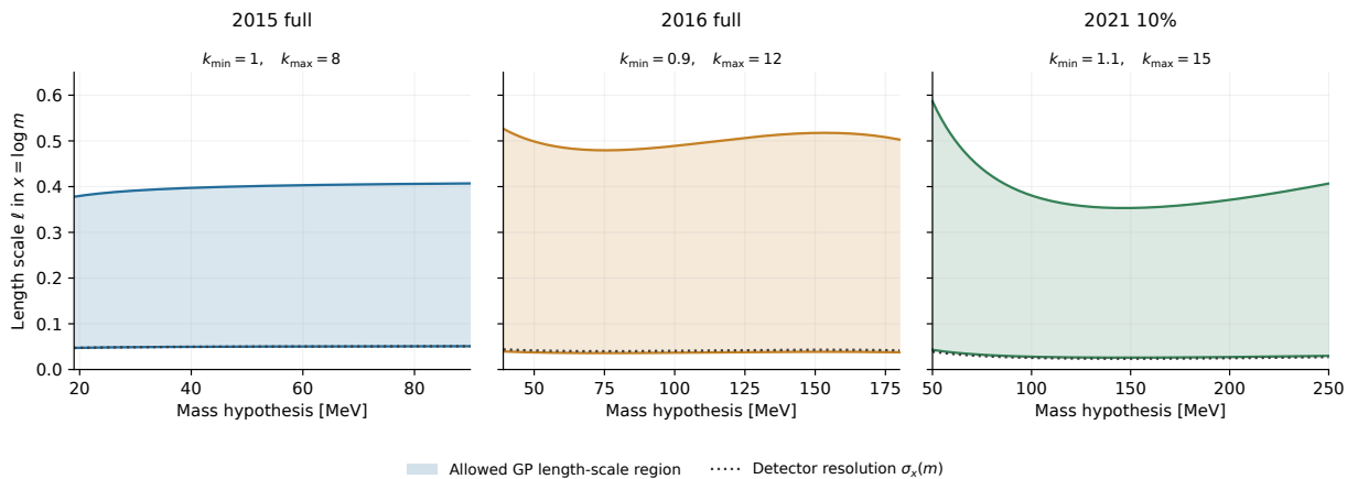
Figure 30: Allowed RBF length scales in x = \log m across the three search ranges. Shading lies between the lower and upper bounds evaluated from the frozen analysis card; the dotted curves show the local detector-resolution scale \sigma_x(m) . The lower/upper factors are 1.0/8, 0.9/12, and 1.1/15 for 2015, 2016, and 2021, respectively. These are numerical domains for the sideband fit, not fitted length scales or detector-resolution uncertainties.
