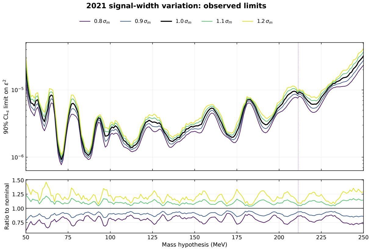
Figure 67: 2021 observed 90% CL s limits for the five signal-template widths, with ratios to the nominal limit below. Every curve uses the same archived GP prediction and yield conversion. The visible-branching correction is common to all curves and cancels in the ratios. The plots retain all 1,005 saved limits.
