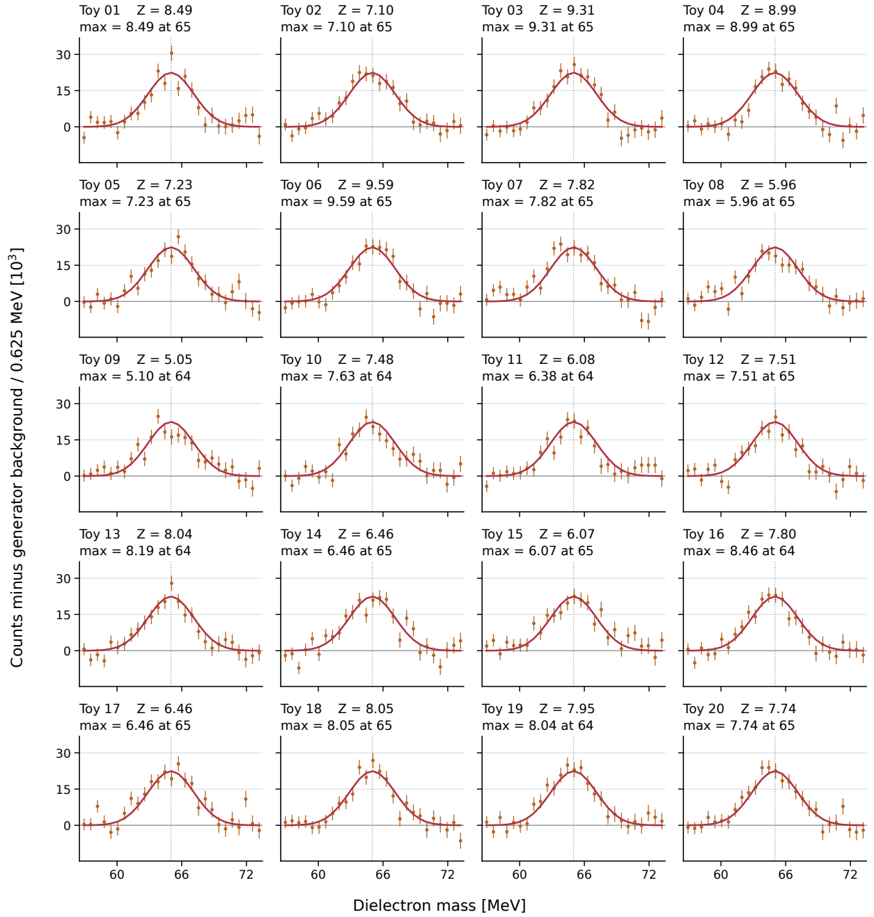
Figure 152: Saved v5.6.0 fit catalogue: 20 Poisson realizations of the 10%-based 65 MeV injection. The panel labels and residual conventions are retained from the standalone study. All draws are shown; none is chosen for resemblance to the data.
