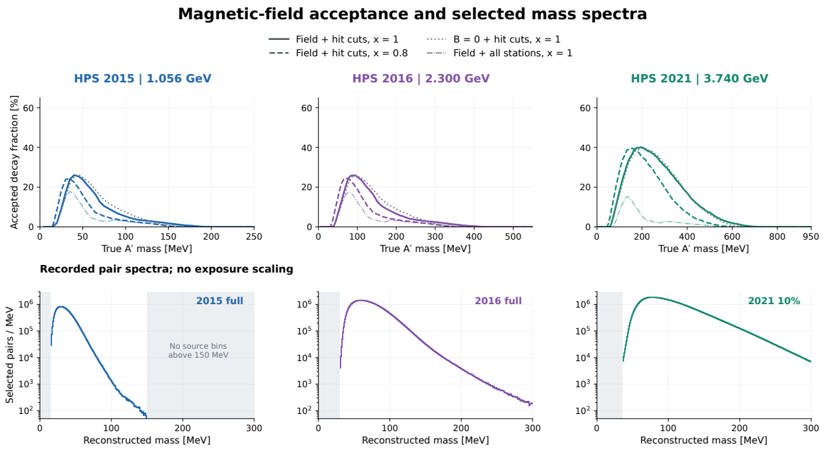
Figure 154: Conditional geometry fractions and the separately measured selected pair spectra. The spectra retain their native exposures and selections; their shapes and integrals are not signal efficiencies or production rates.
