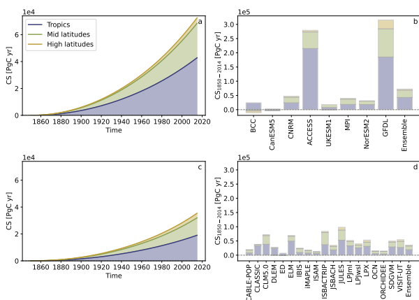
Figure 3 Temporal trends in Carbon Sequestration (CS) (a,c) and CS at the end of the period from 1850 to 2014 (b,d) calculated using NEP from CMIP6 (a,b) and TRENDY (c,d) and the contributions of latitudinal zones (colors). Panels a and c show results from the CMIP6 and TRENDY models' average ensemble, respectively, and panels b and d show results for each model alongside the ensemble. The dotted lines represent null CS values, with negative (positive) values indicating carbon debts (surpluses). To optimize space, only the initial part of each model name is displayed on the horizontal axes in b.
