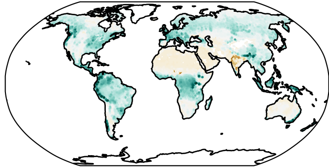
c) X-BASE
