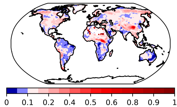
MOHC
