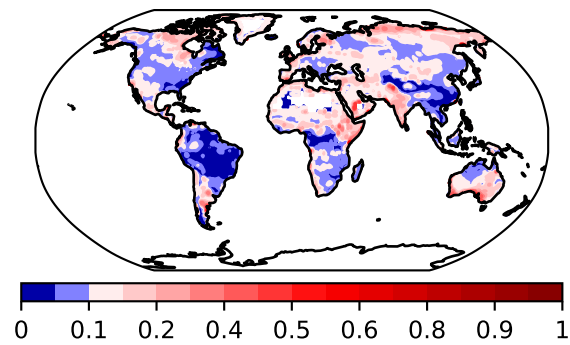
NCAR
