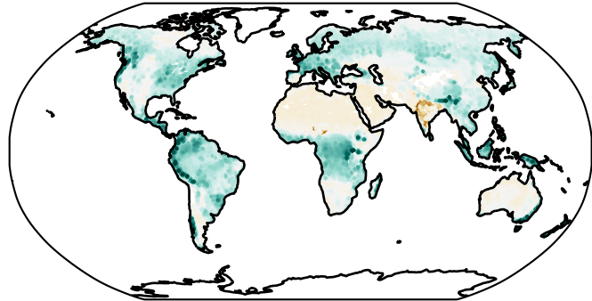
c) FLUXCOM-X
