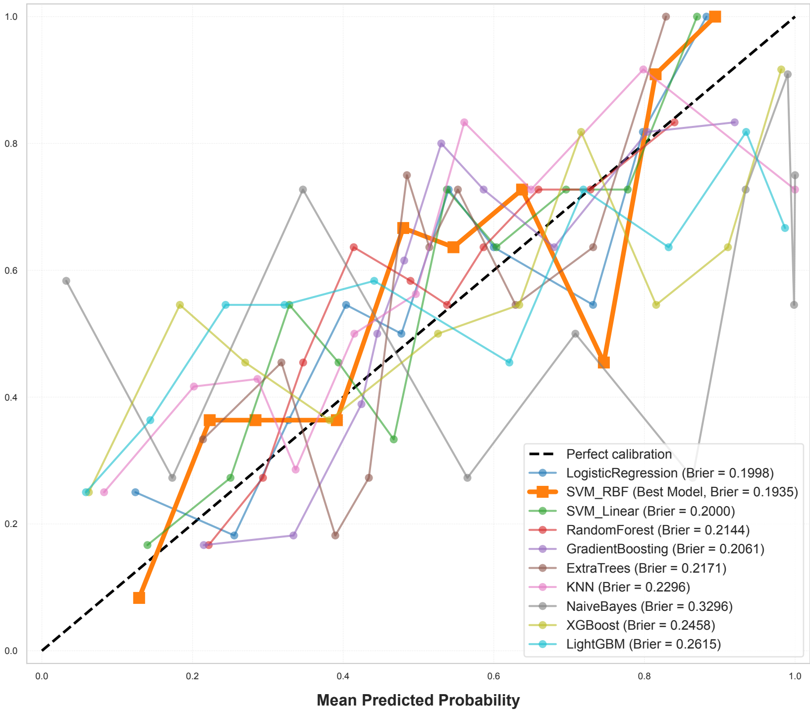
Calibration Curves (Quantile Binning)
