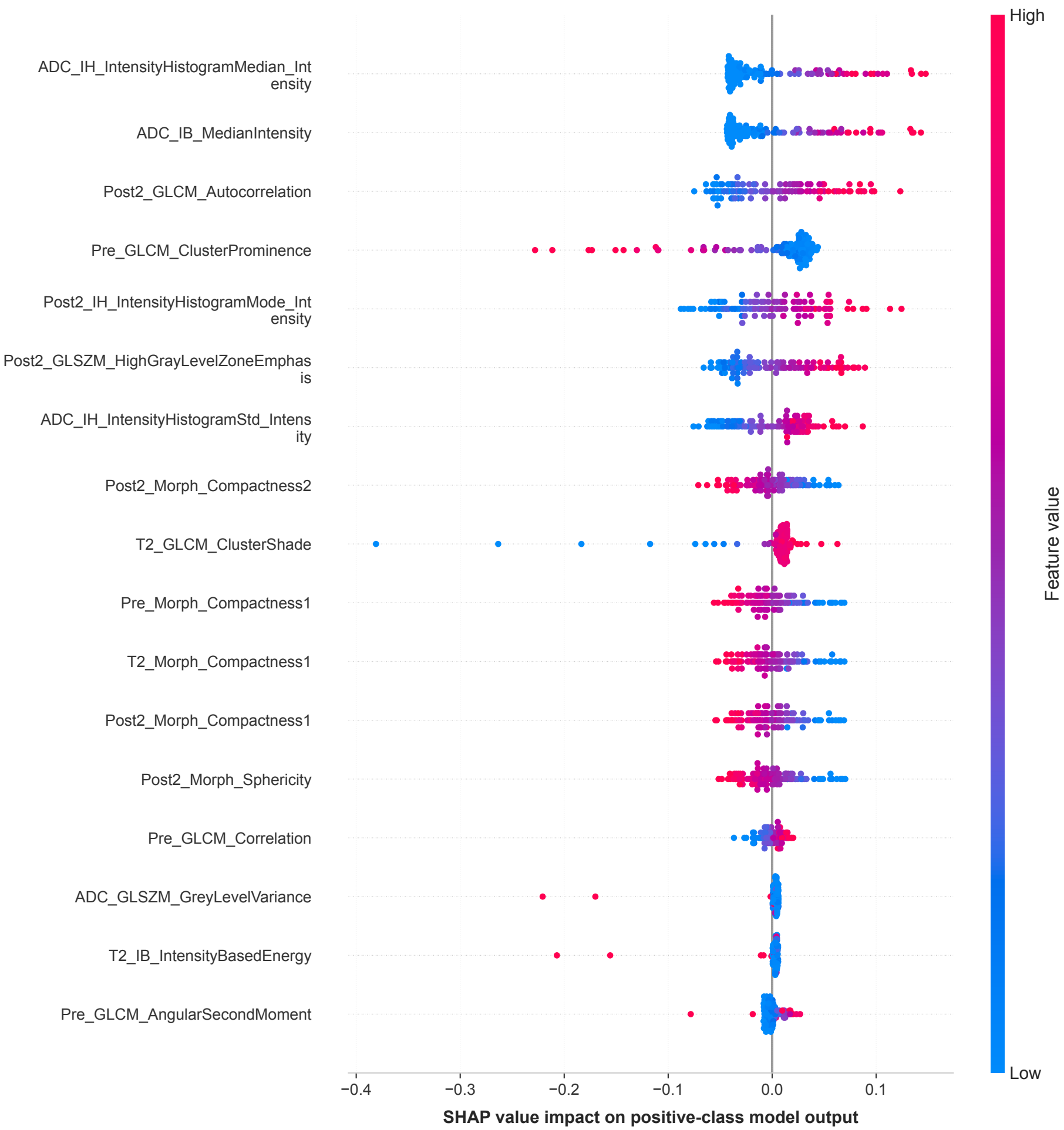
SHAP Summary Plot Model: SVM_RBF | OOF AUC: 0.737 | OOF Kappa: 0.351
