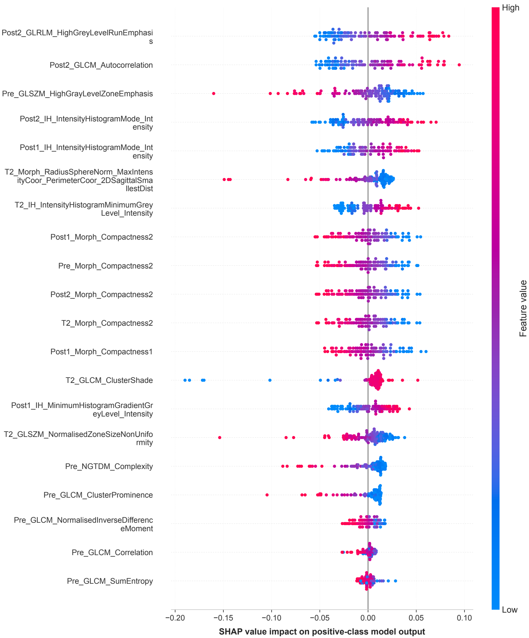
SHAP Summary Plot Model: SVM_RBF | OOF AUC: 0.713 | OOF Kappa: 0.326
