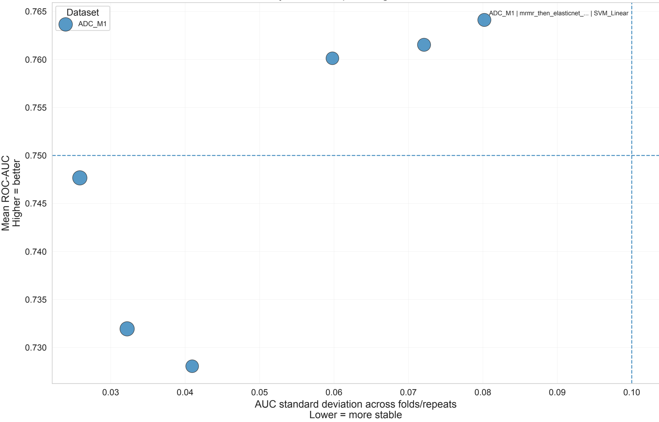
Performance–Stability Pareto Map of Single-Dataset Radiomics Models
