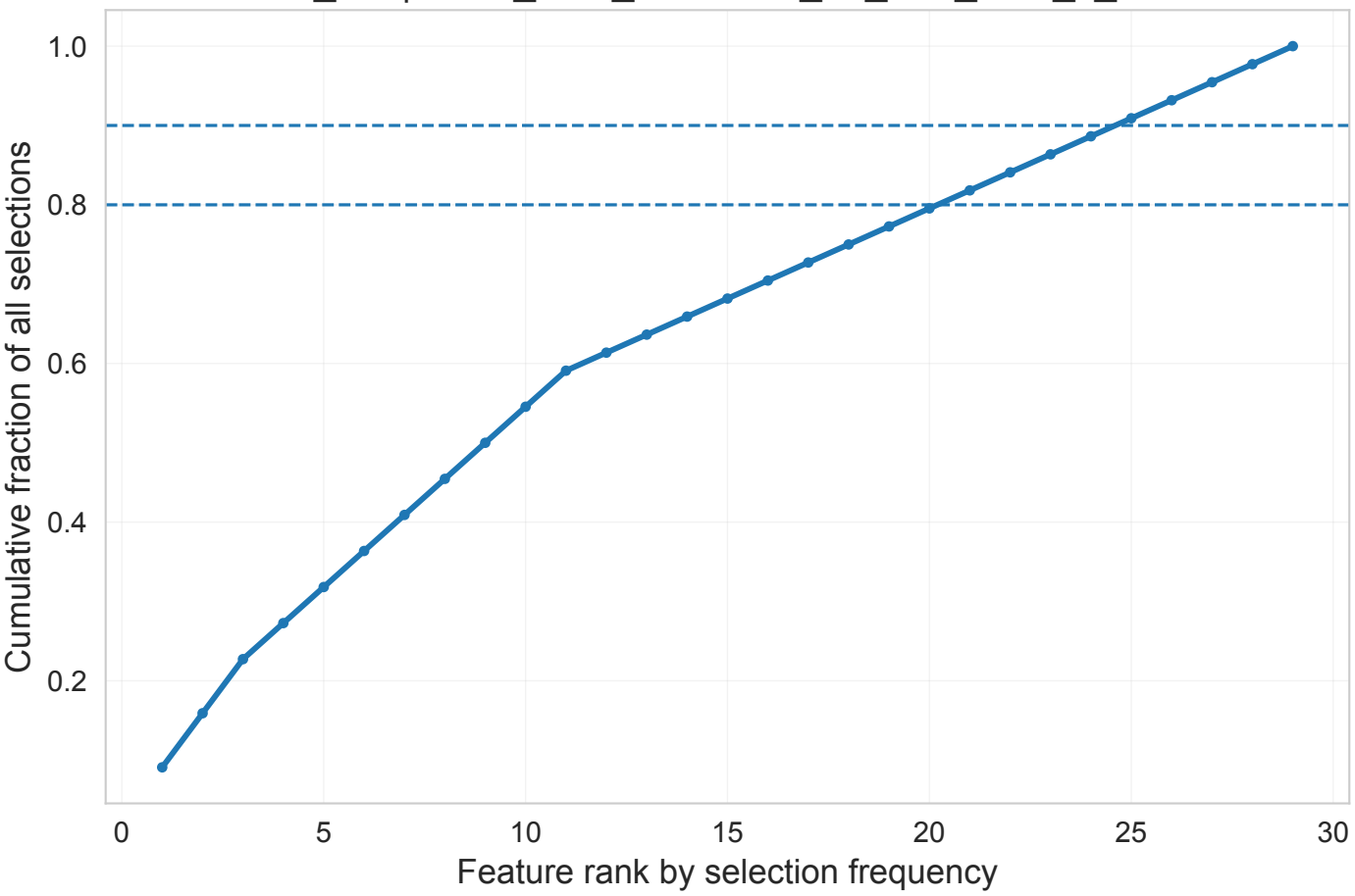
Cumulative Feature Selection Concentration ADC_M1 | mrmr_then_elasticnet_no_corr_auto_k_smote
