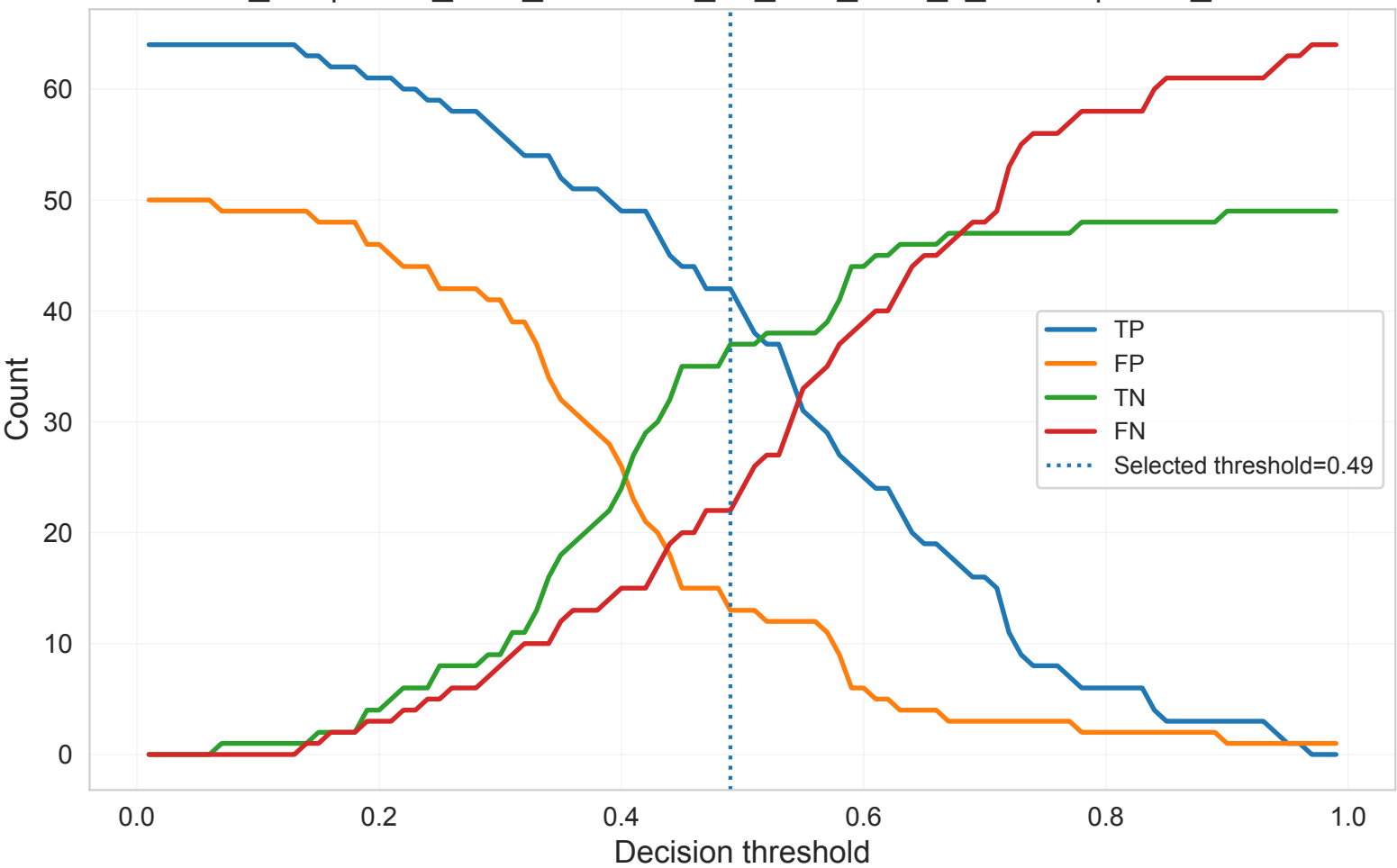
Confusion-Count Dynamics Across Thresholds ADC_M1 | mrmr_then_elasticnet_no_corr_auto_k_smote | SVM_Linear
