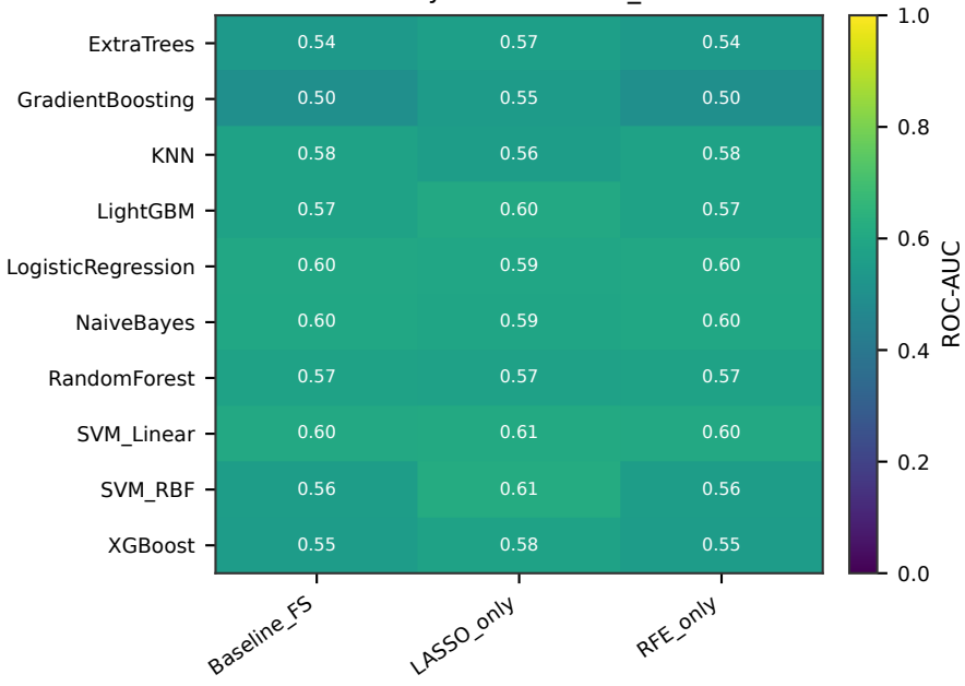
ROC-AUC by Model and FS_METHOD
