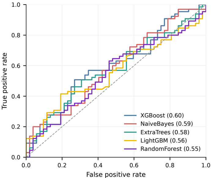
Baseline ROC Curves
