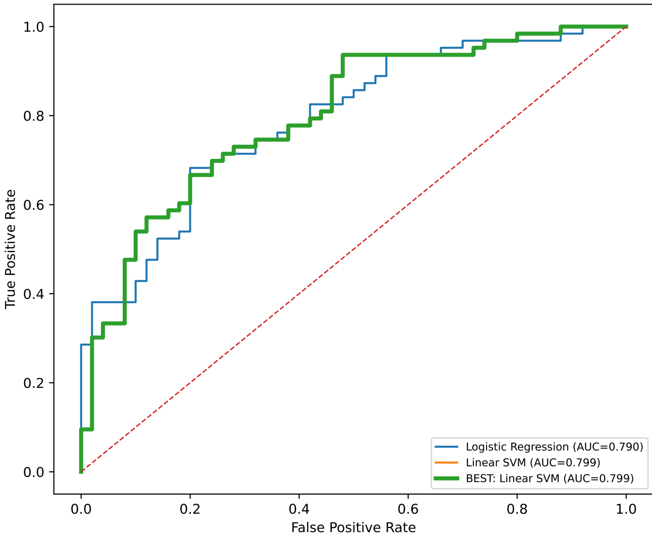
ROC Curves - ADC Post1 Pre Fusion
