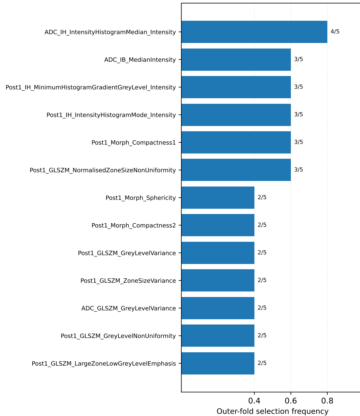
Feature-selection recurrence
