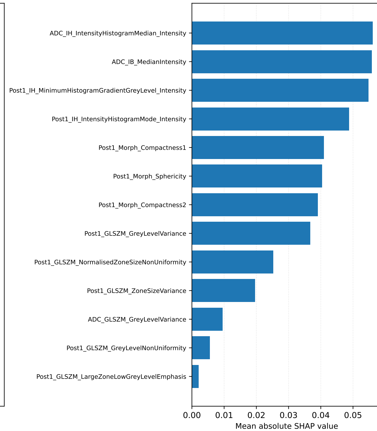
Global SHAP importance
