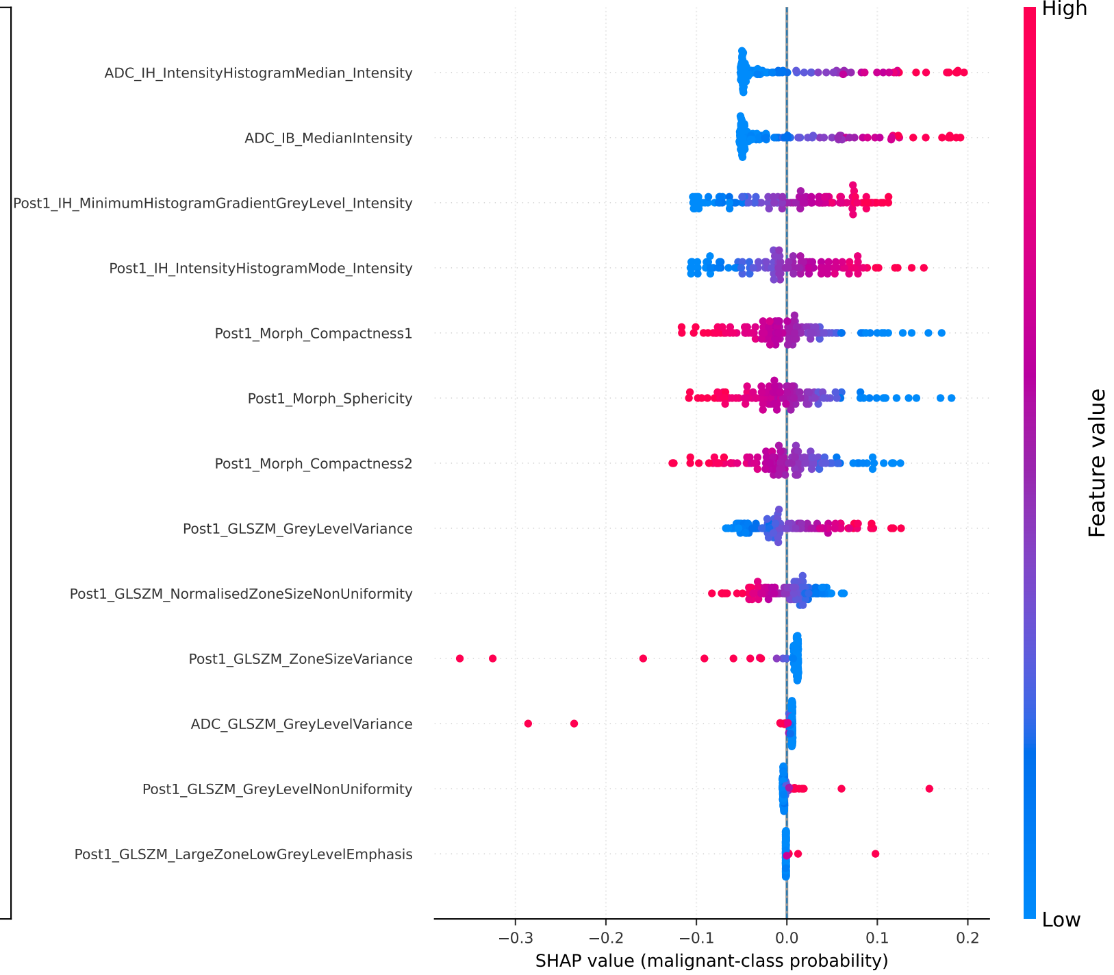
SHAP summary
