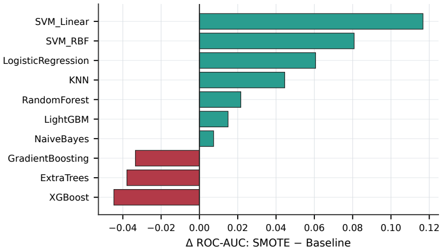
Effect of SMOTE on ROC-AUC
