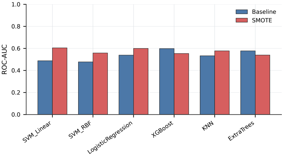
ROC-AUC Before and After SMOTE
