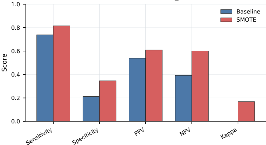
Metric Trade-off — SVM_Linear
