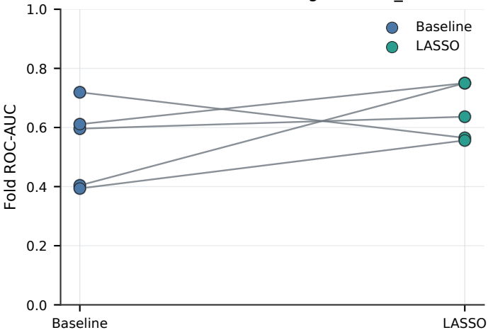
Outer-fold ROC-AUC Change — SVM_Linear
