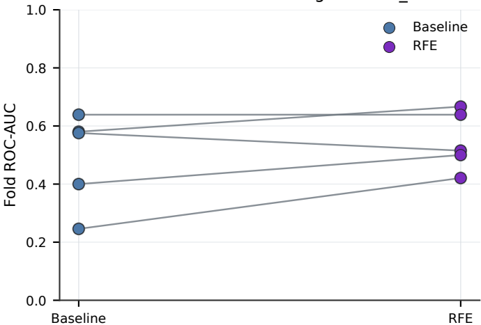
Outer-fold ROC-AUC Change — SVM_RBF
