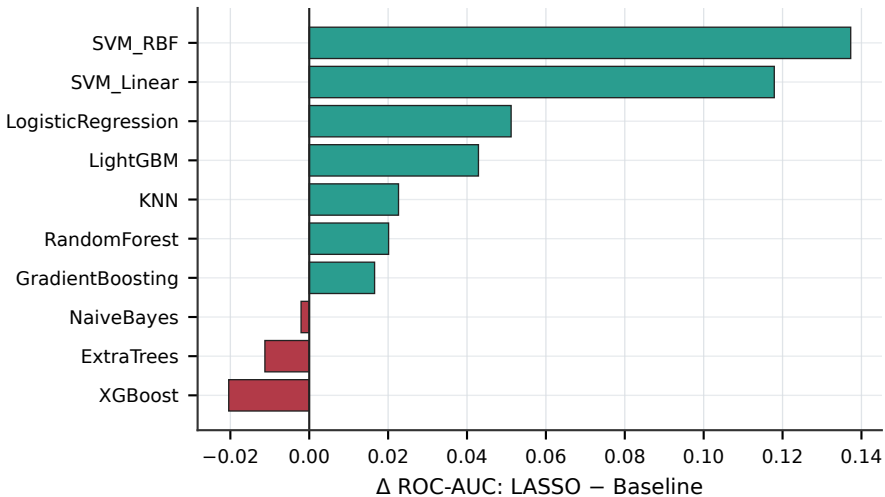
Effect of LASSO Feature Selection
