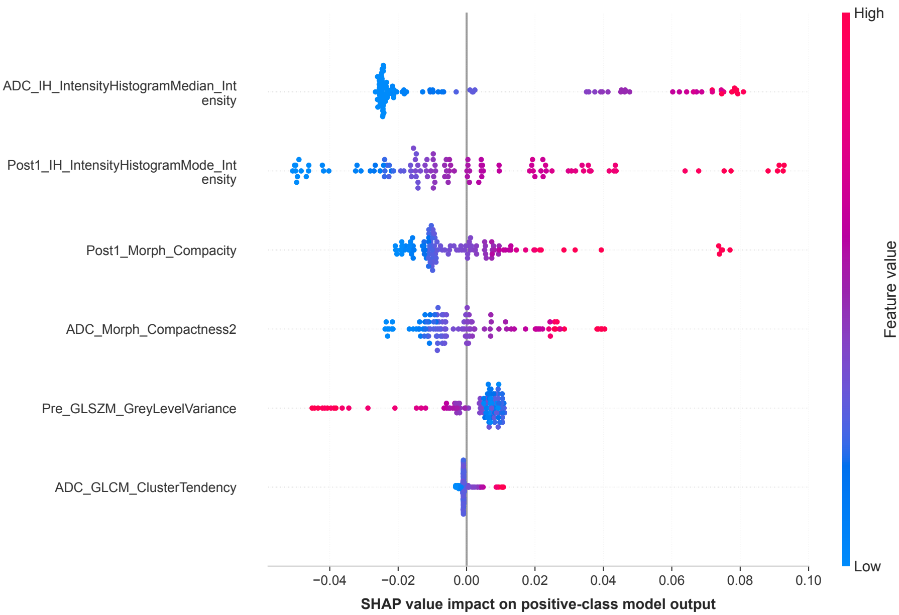
SHAP Summary Plot Model: ExtraTrees | OOF AUC: 0.729 | OOF Kappa: 0.362
