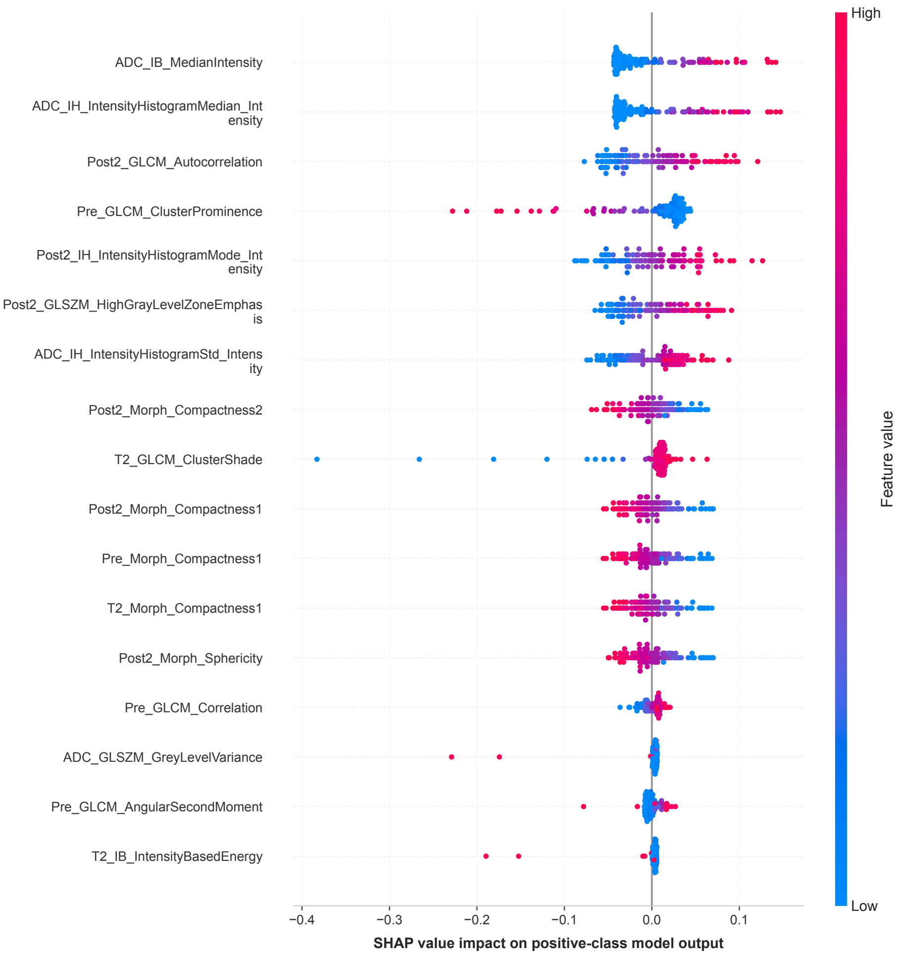
SHAP Summary Plot Model: SVM_RBF | OOF AUC: 0.723 | OOF Kappa: 0.350
