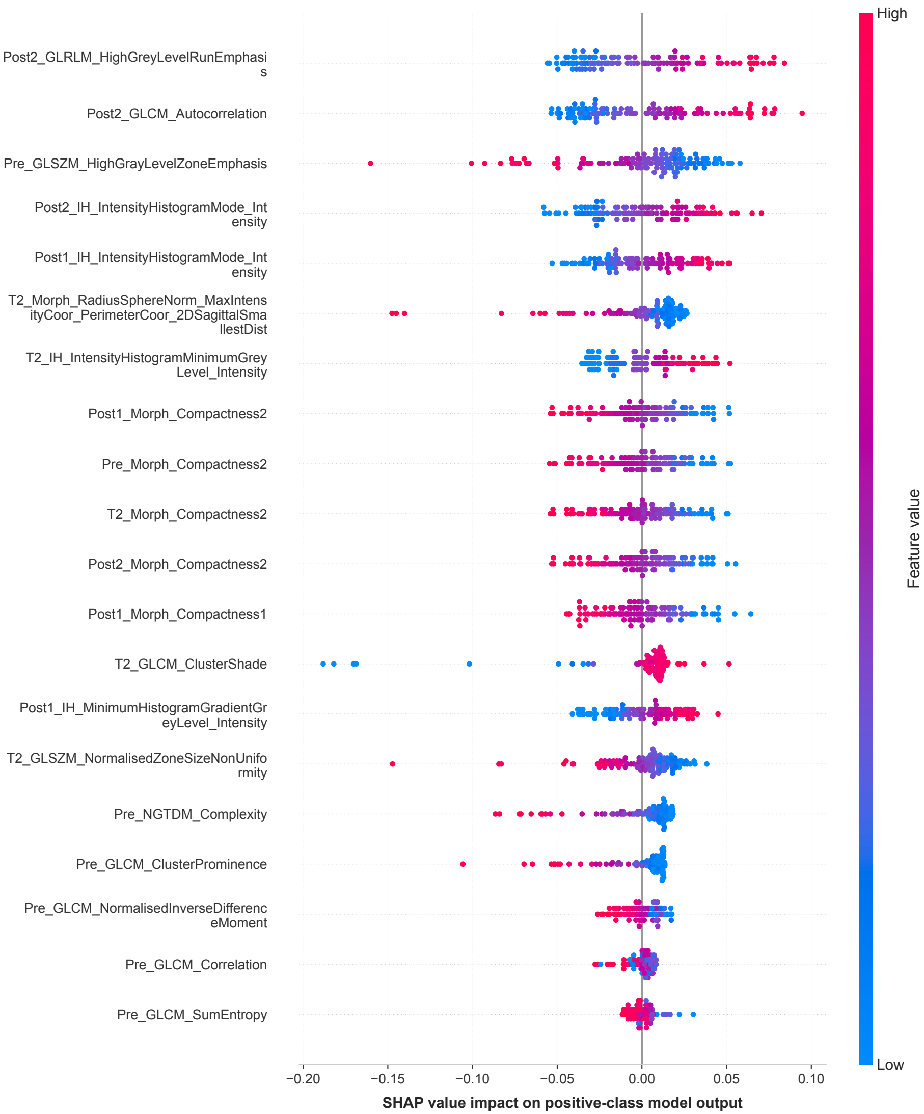
SHAP Summary Plot Model: SVM_RBF | OOF AUC: 0.659 | OOF Kappa: 0.178
