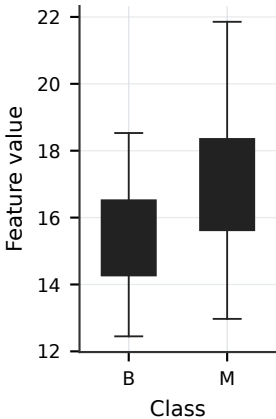
Post1_Morph_CompactnessPost1_Morph_CompactnessPost1_Morph_CompactnessPost1_Morph_SphericalID
