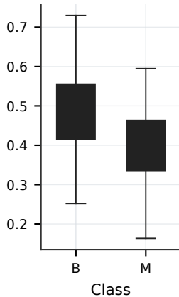
Post1_Morph_CompactnessPost1_Morph_CompactnessPost1_Morph_CompactnessPost1_Morph_SphericalID
