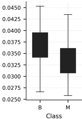
Post1_Morph_CompactnessPost1_Morph_CompactnessPost1_Morph_CompactnessPost1_Morph_SphericalID
