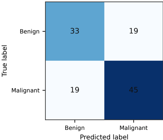
Confusion Matrix — ExtraTrees
