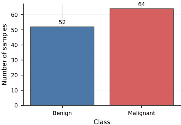
Class Distribution
