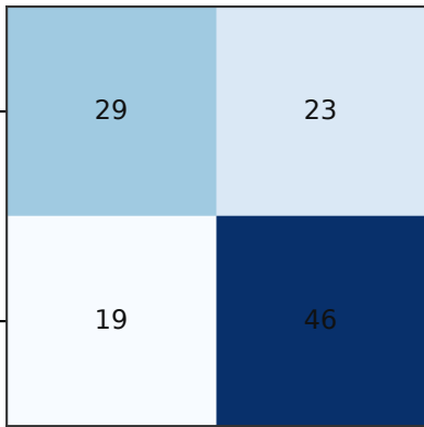
Confusion Matrix — XGBoost
