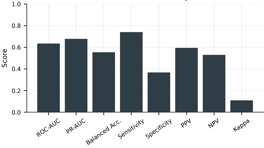
Metric Profile — NaiveBayes
