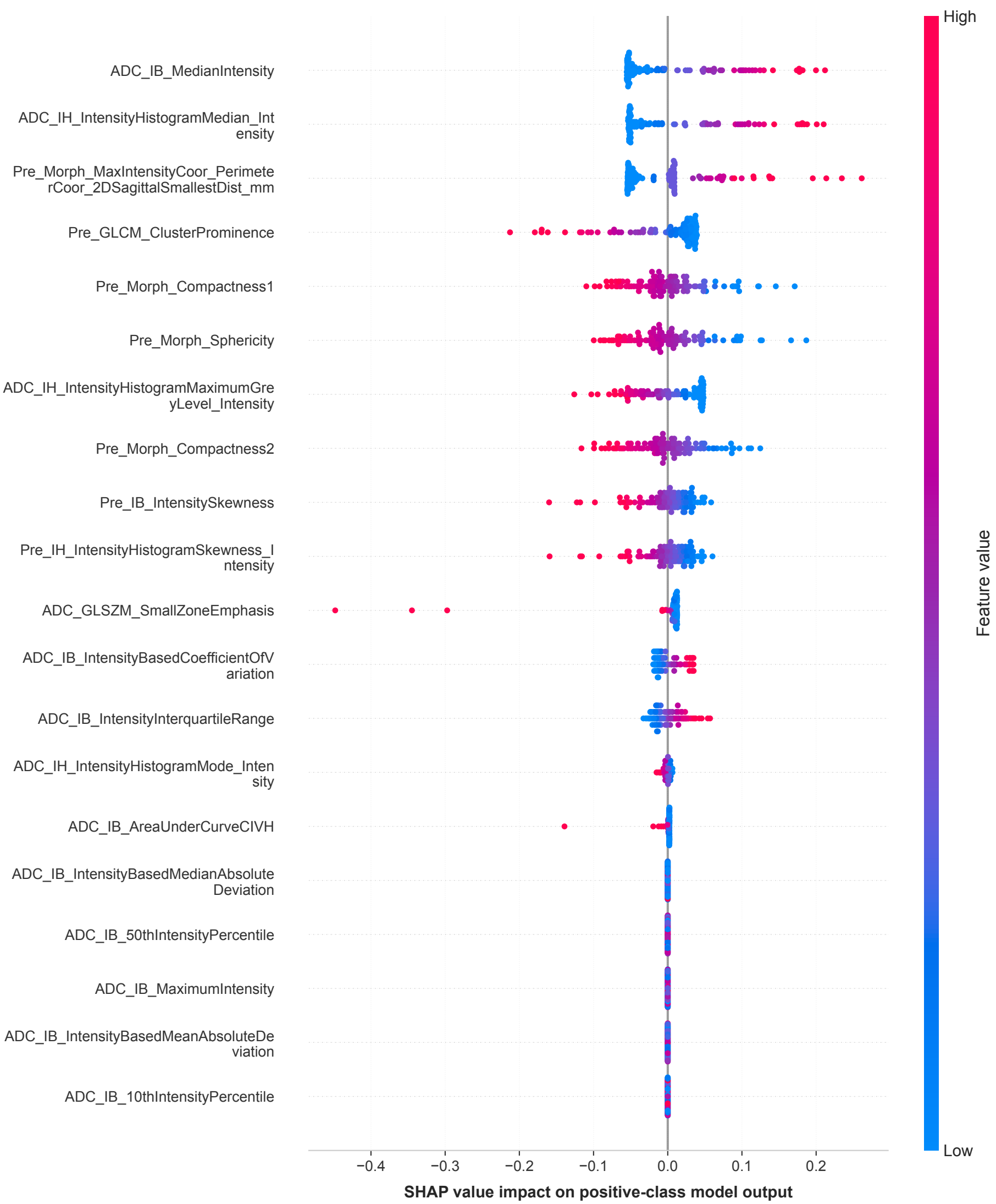
SHAP Summary Plot Model: LogisticRegression | OOF AUC: 0.686 | OOF Kappa: 0.332
