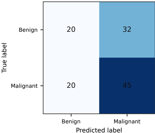
Confusion Matrix — NaiveBayes
