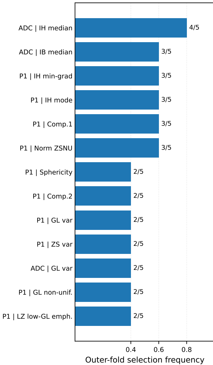
(a) Feature-selection recurrence
