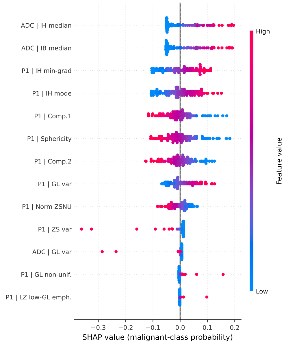
(c) SHAP summary
