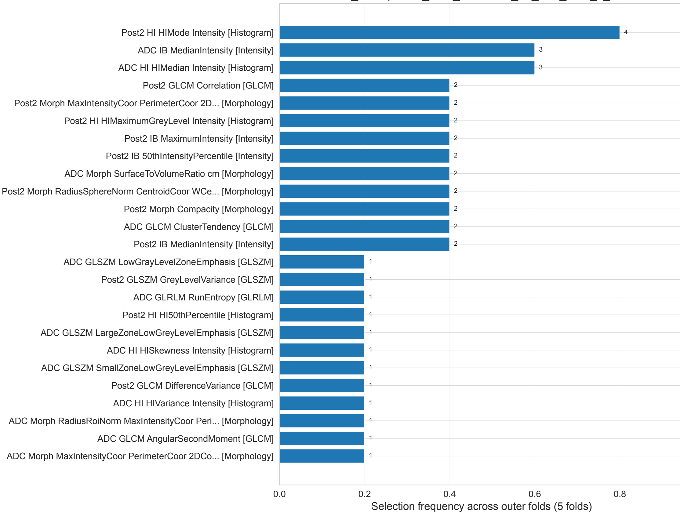
Most Stable Selected Radiomics Features Post2_ADC | mrmr_then_elasticnet_no_corr_auto_k_smote
