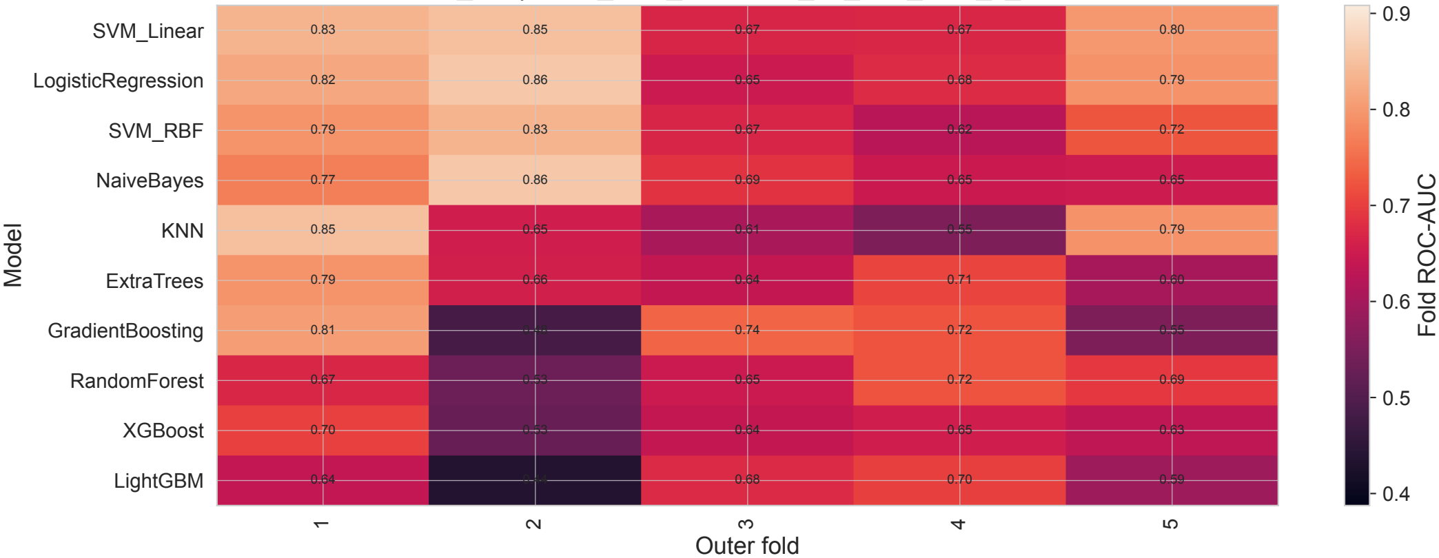
Fold-Level ROC-AUC Failure Map ADC_M1 | mrmr_then_elasticnet_no_corr_auto_k_smote
