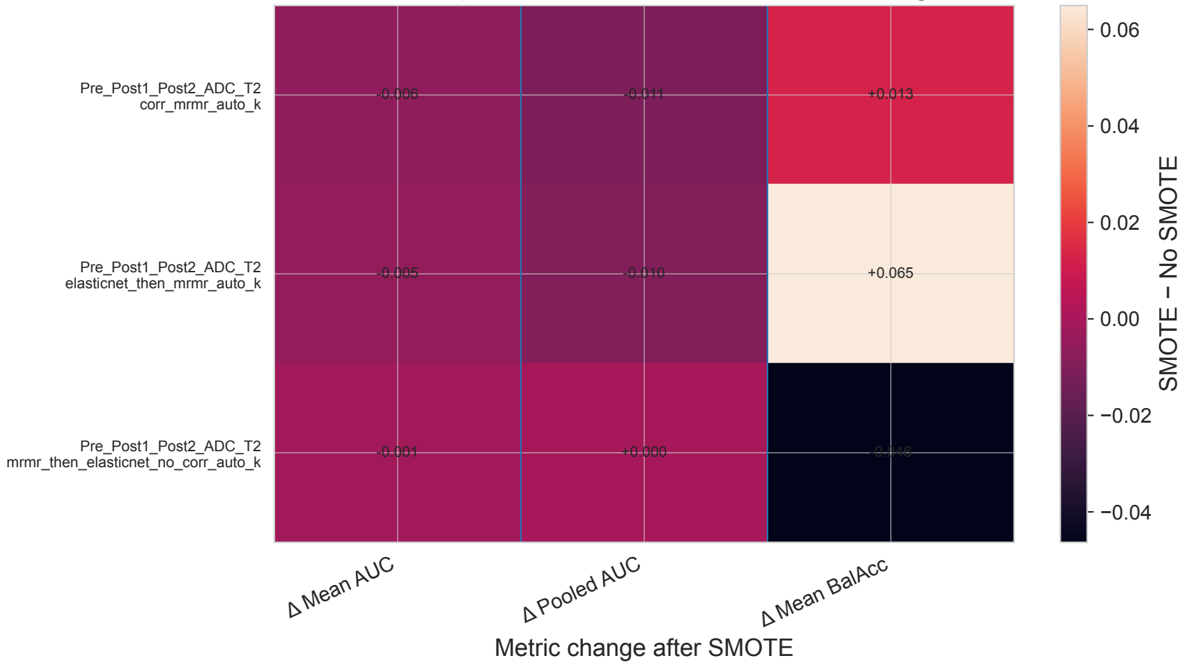
SMOTE Impact Across Feature-Selection Strategies
