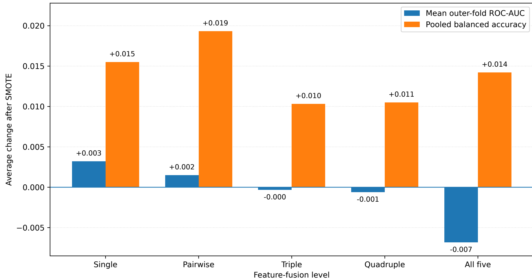
Average effect of SMOTE by feature-fusion level
