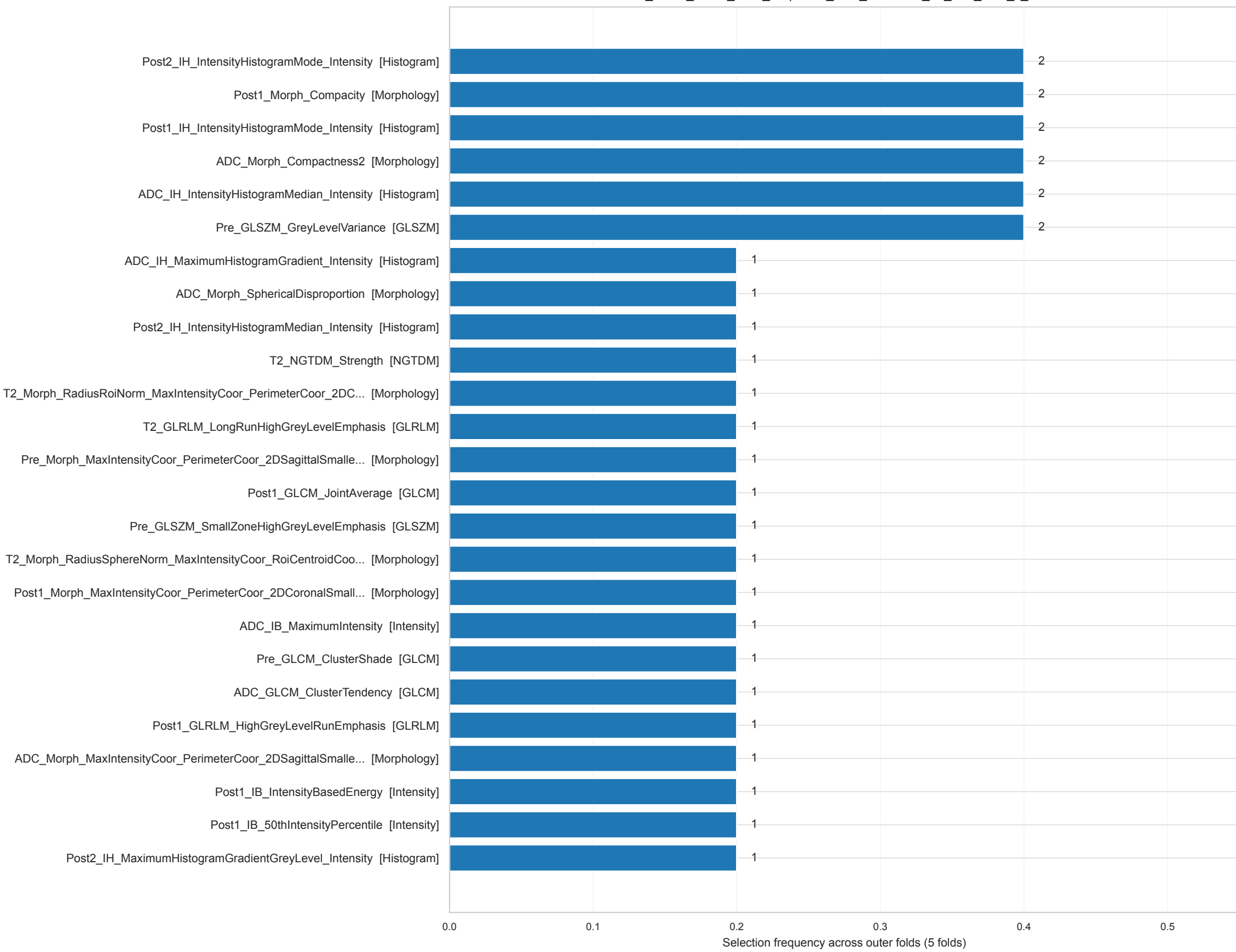
Most Stable Selected Radiomics Features Pre_Post1_Post2_ADC_T2 | mrmr_then_elasticnet_no_corr_auto_k_smote
