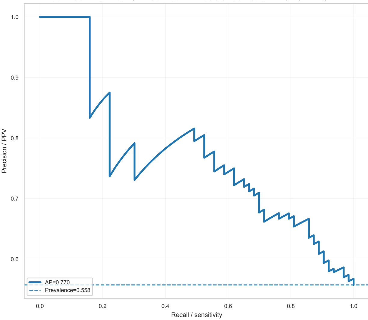
Precision-Recall Curve Pre_Post1_Post2_ADC_T2 | mrmr_then_elasticnet_no_corr_auto_k_smote | LogisticRegression
