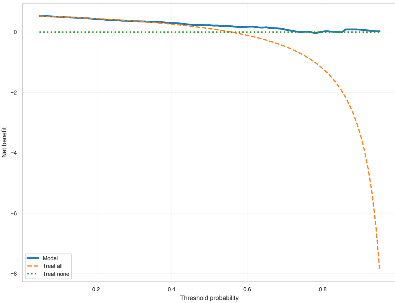
Decision Curve Analysis Pre_Post1_Post2_ADC_T2 | mrmr_then_elasticnet_no_corr_auto_k_smote | LogisticRegression
