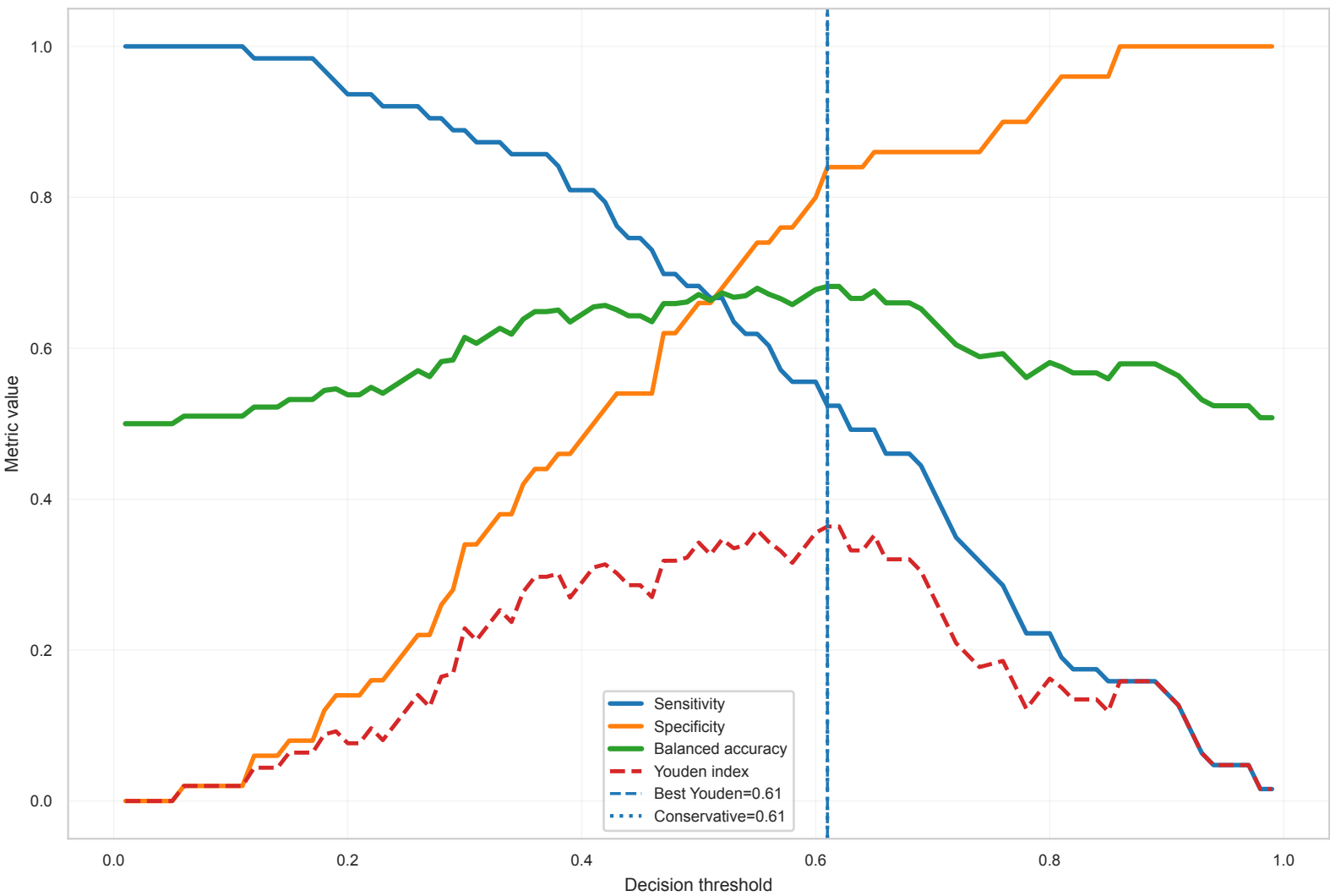
Threshold Operating Characteristic Pre_Post1_Post2_ADC_T2 | mmmr_then_elasticnet_no_corr_auto_k_smote | LogisticRegression
