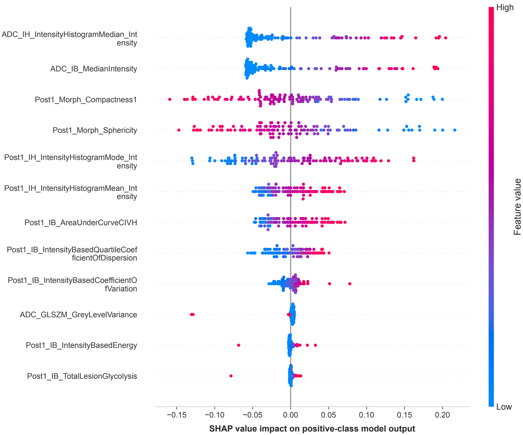
SHAP Summary Plot Model: SVM_RBF | OOF AUC: 0.783 | OOF Kappa: 0.433
