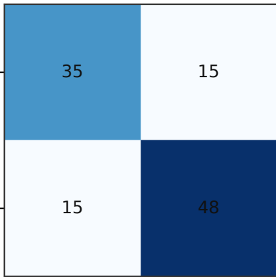
Confusion Matrix — SVM_RBF
