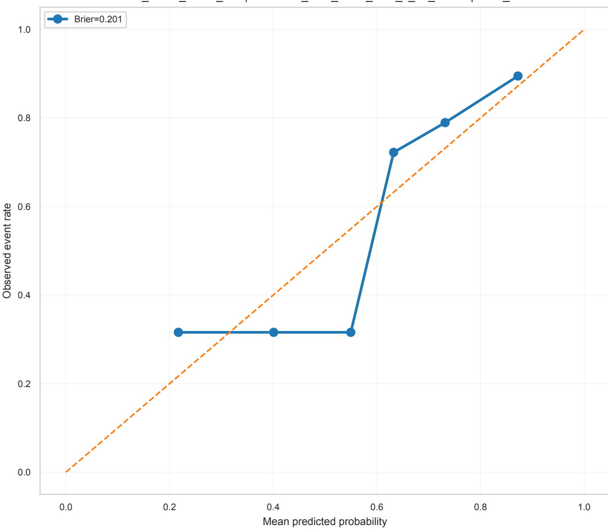
Calibration Curve ADC_Post1_Post2_Pre | elasticnet_then_mrrmr_auto_k_no_smote | SVM_RBF
