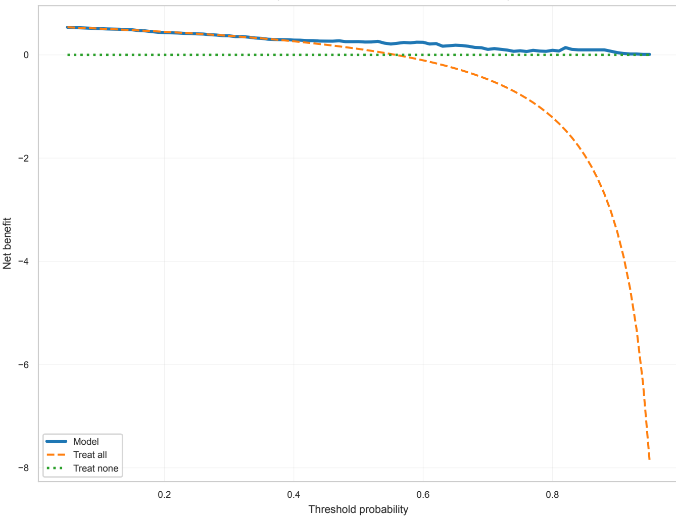
Decision Curve Analysis ADC_Post1_Post2_Pre | elasticnet_then_mrmr_auto_k_no_smote | SVM_RBF
