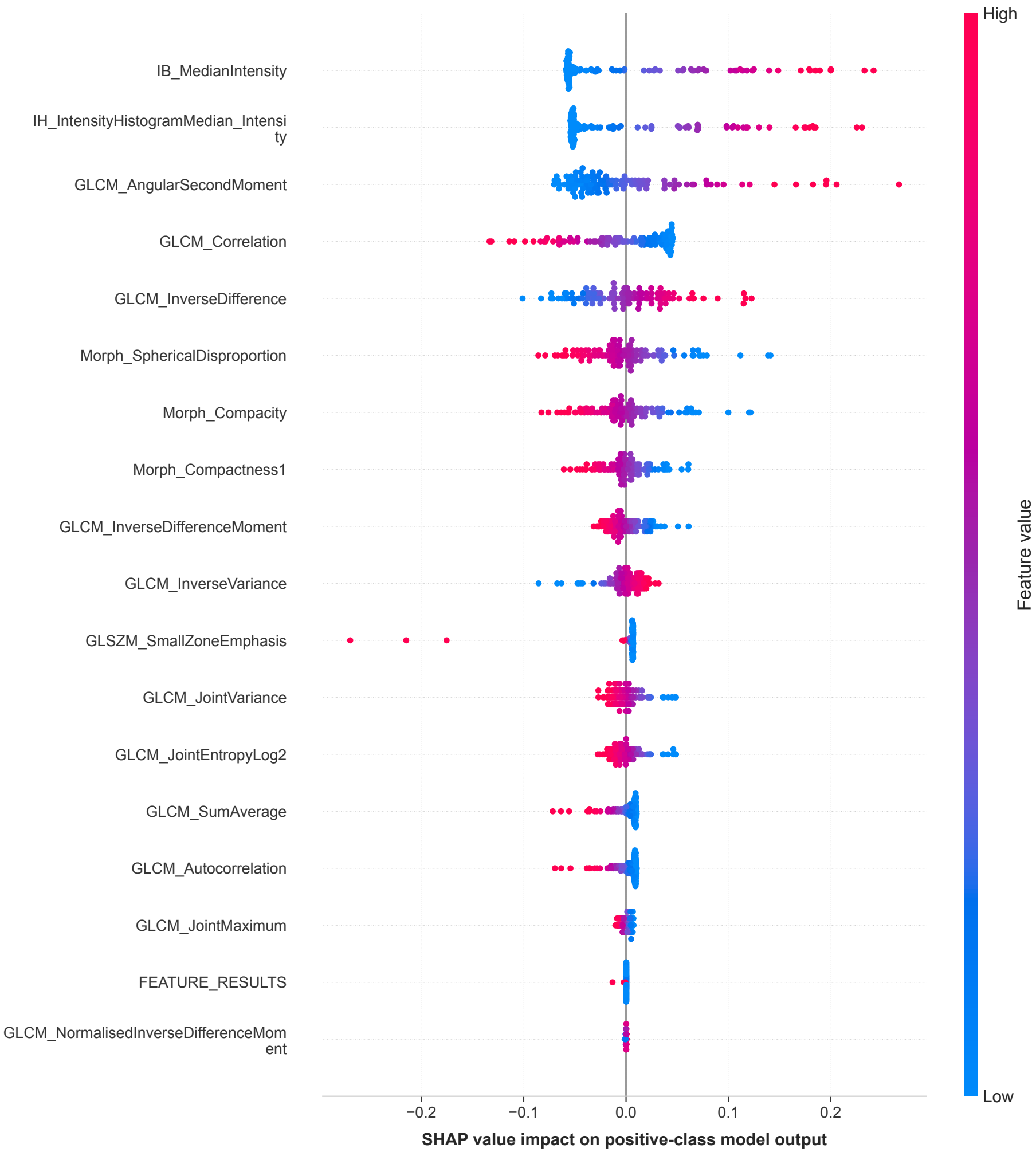
SHAP Summary Plot Model: SVM_Linear | OOF AUC: 0.720 | OOF Kappa: 0.372
