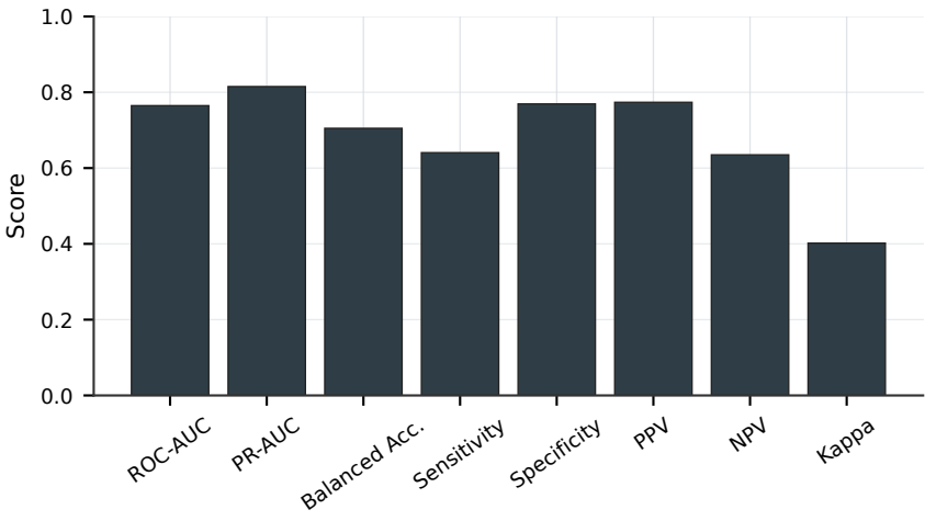
Metric Profile — KNN
