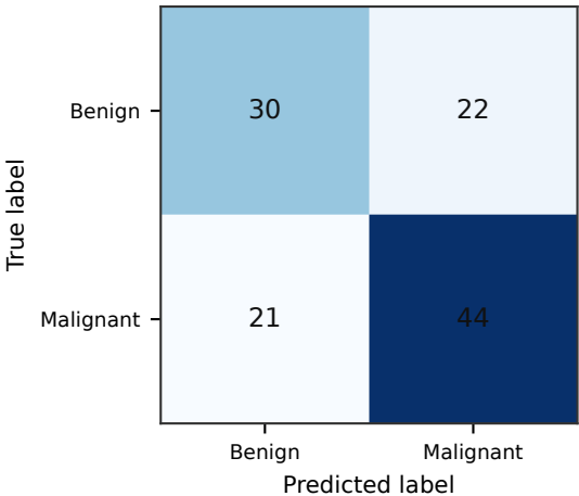
Confusion Matrix — GradientBoosting
