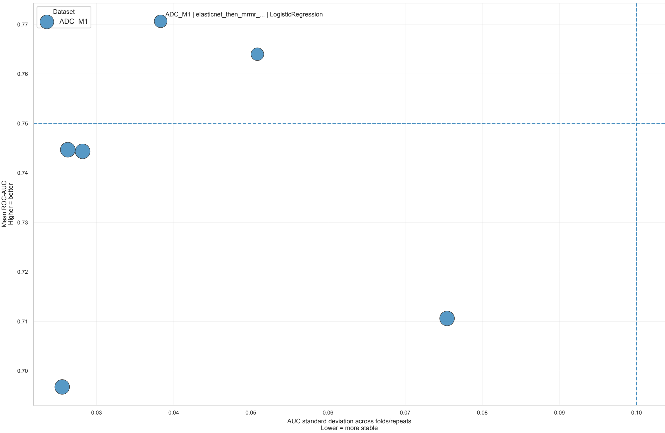
Performance–Stability Pareto Map of Single-Dataset Radiomics Models
