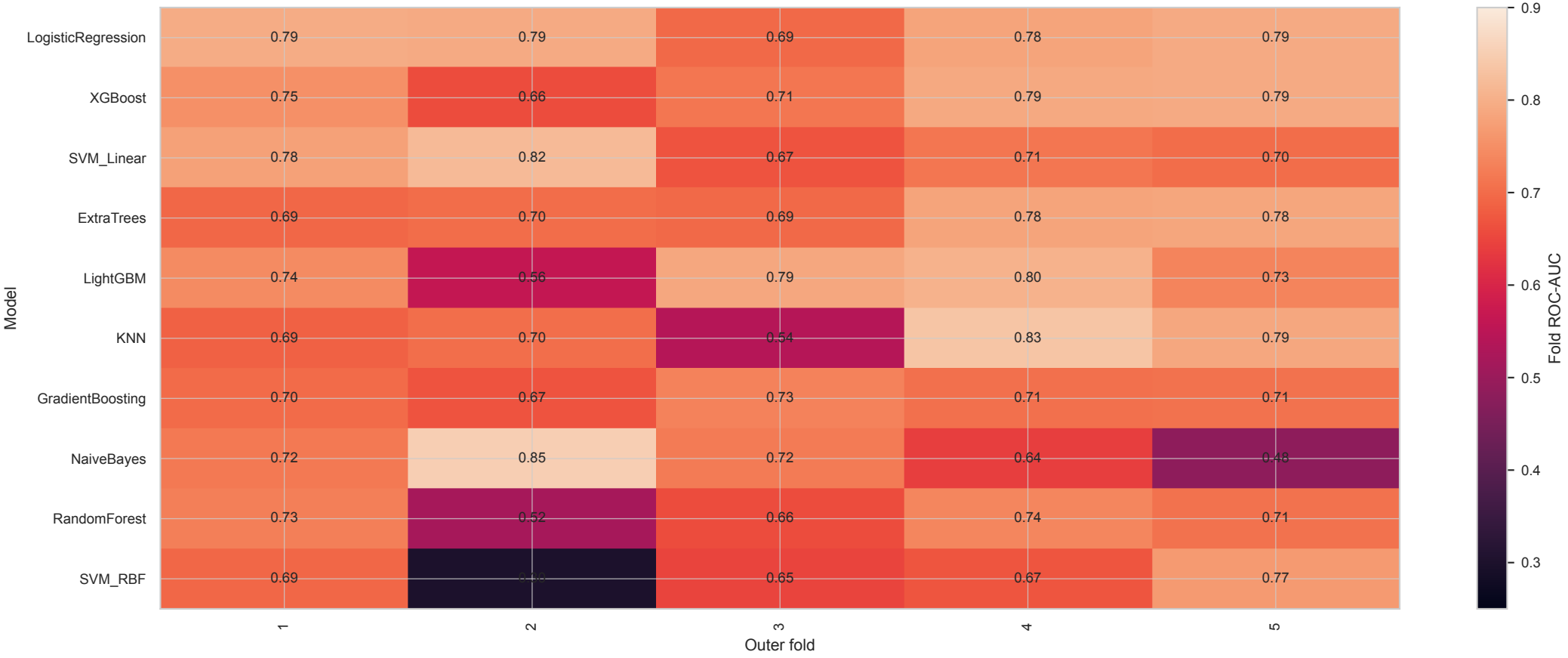
Fold-Level ROC-AUC Failure Map ADC_M1 | elasticnet_then_mrmr_auto_k_no_smote
